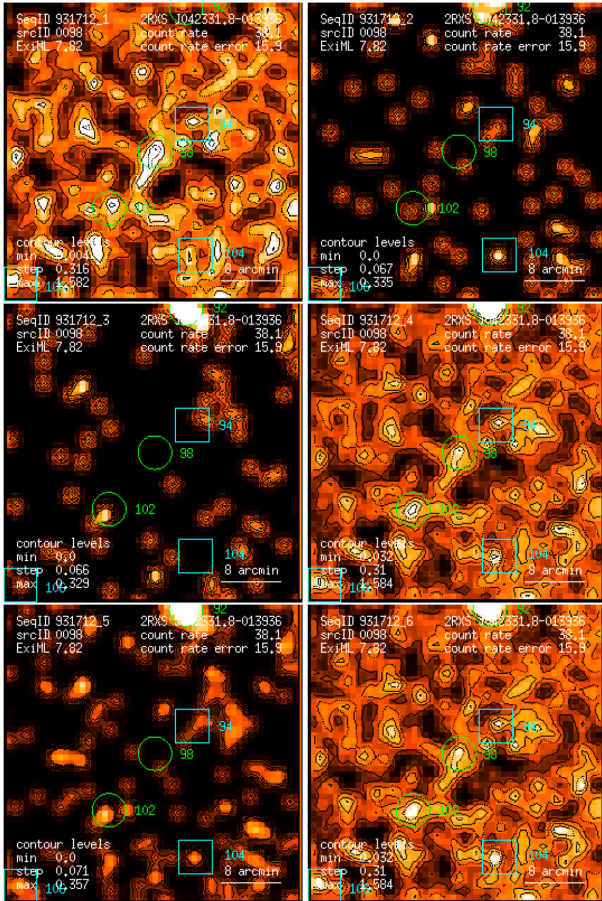
Figure 98: RASS 931712: detection 0098: band rate images, Gaussian filter: (1) PSPC channels 11 – 41, (2) 52 – 90, (3) 91 – 201, (4) 11 – 235, (5) 52 – 201, (6) 11 – 201. Broad band rates in counts/ks. Band rate contour levels in counts/ks/arcmin 2 .
