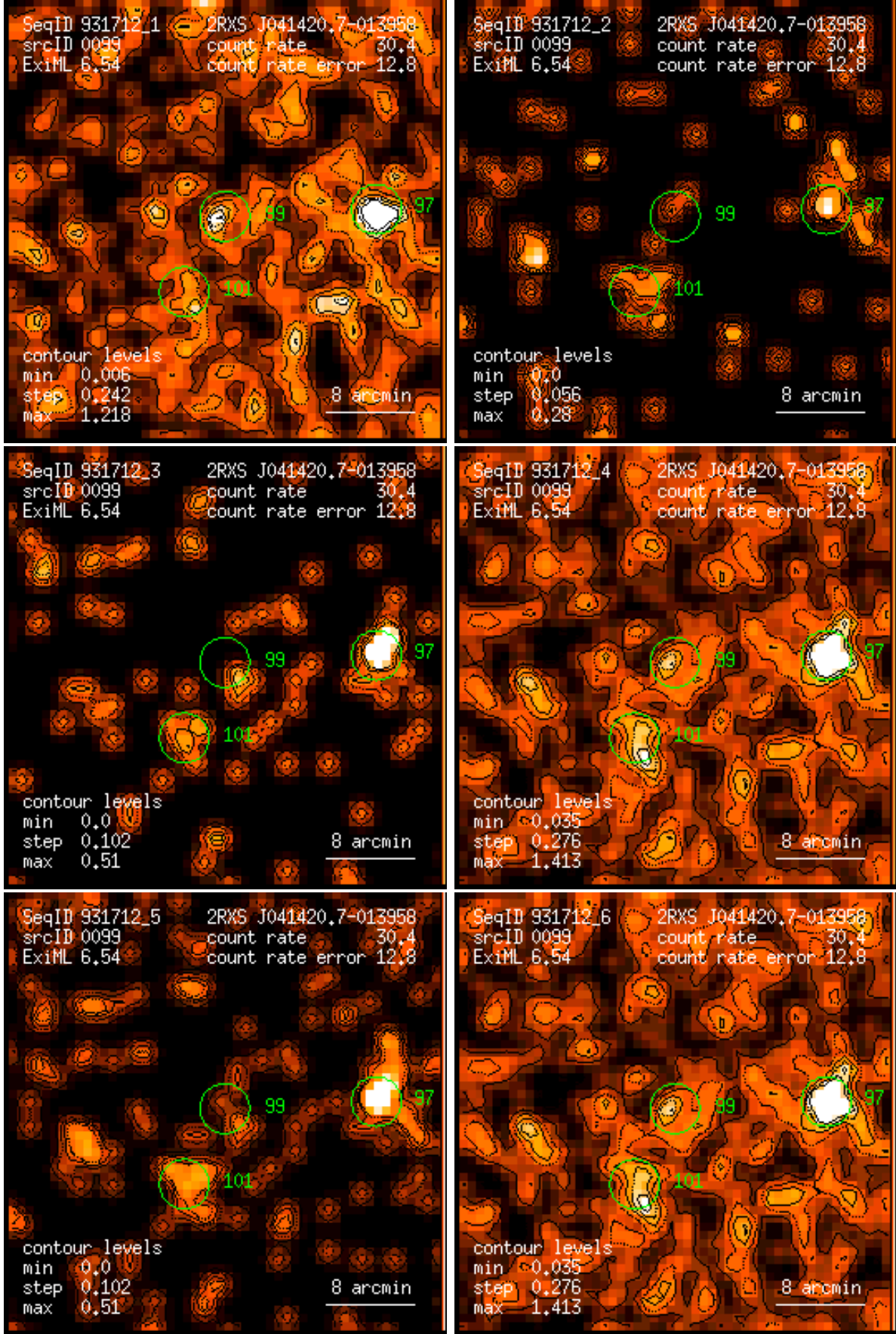
Figure 99: RASS 931712: detection 0099: band rate images, Gaussian filter: (1) PSPC channels 11 – 41, (2) 52 – 90, (3) 91 – 201, (4) 11 – 235, (5) 52 – 201, (6) 11 – 201. Broad band rates in counts/ks. Band rate contour levels in counts/ks/arcmin 2 .
