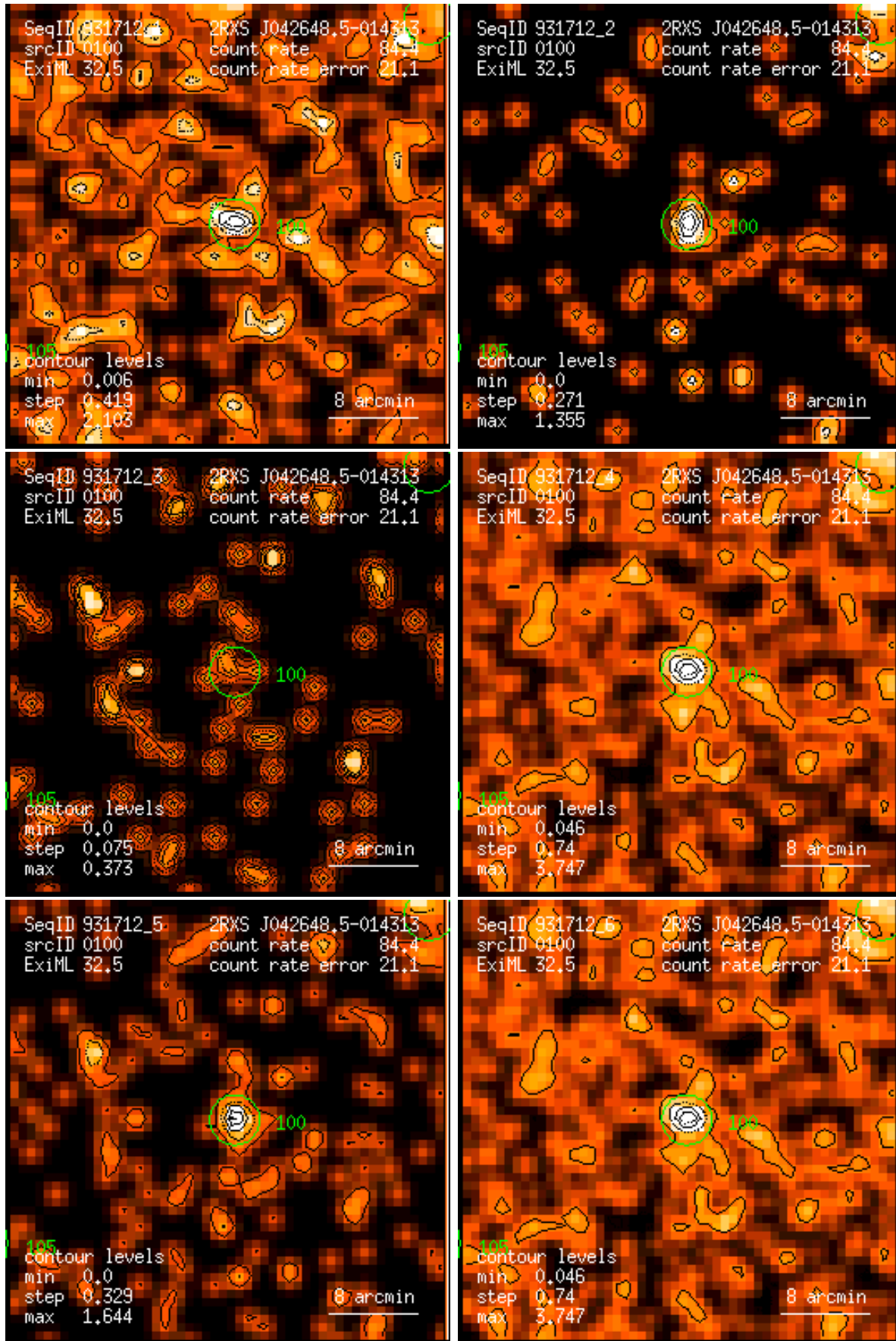
Figure 100: RASS 931712: detection 0100: band rate images, Gaussian filter: (1) PSPC channels 11 – 41, (2) 52 – 90, (3) 91 – 201, (4) 11 – 235, (5) 52 – 201, (6) 11 – 201. Broad band rates in counts/ks. Band rate contour levels in counts/ks/arcmin 2 .
