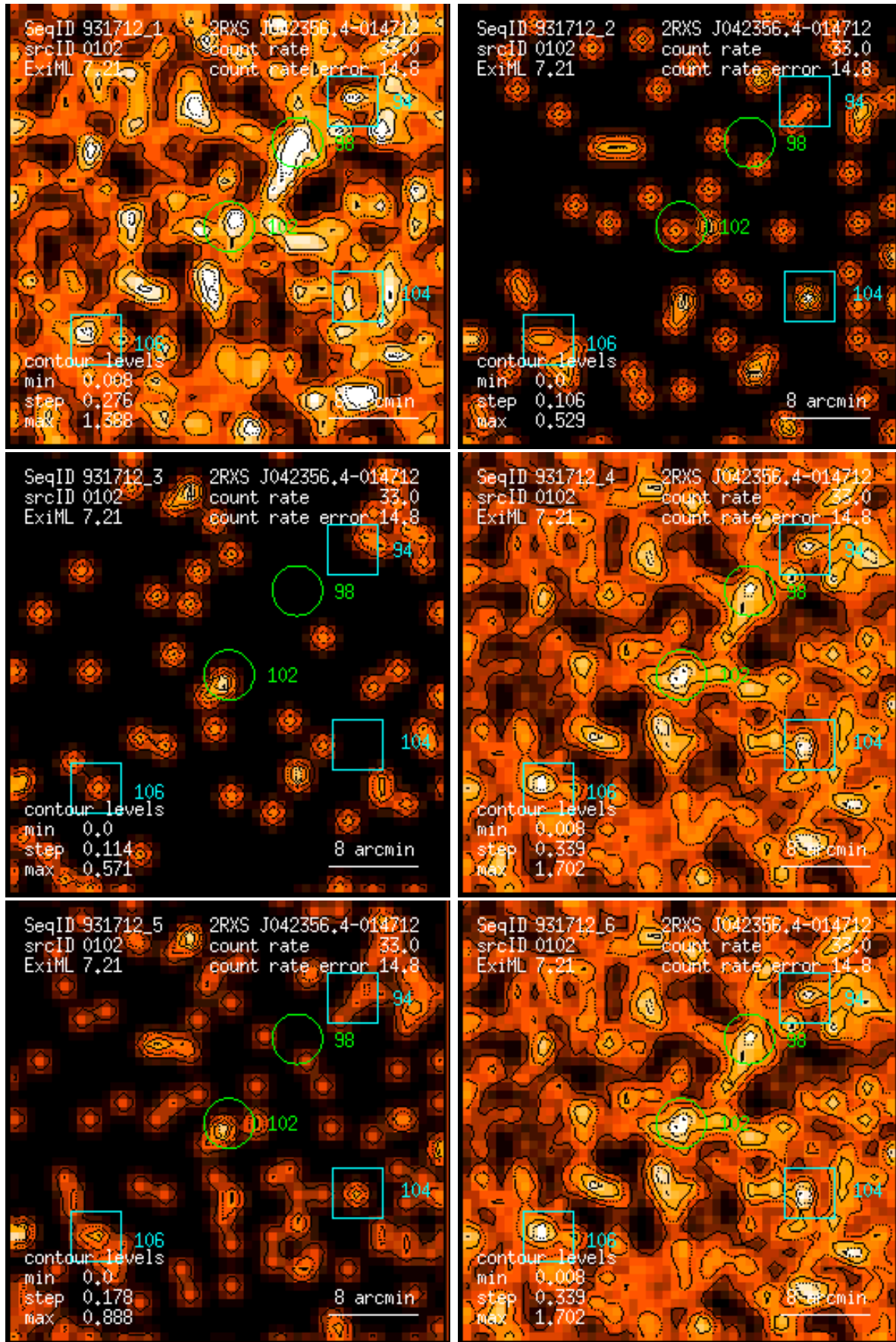
Figure 102: RASS 931712: detection 0102: band rate images, Gaussian filter: (1) PSPC channels 11 – 41, (2) 52 – 90, (3) 91 – 201, (4) 11 – 235, (5) 52 – 201, (6) 11 – 201. Broad band rates in counts/ks. Band rate contour levels in counts/ks/arcmin 2 .
