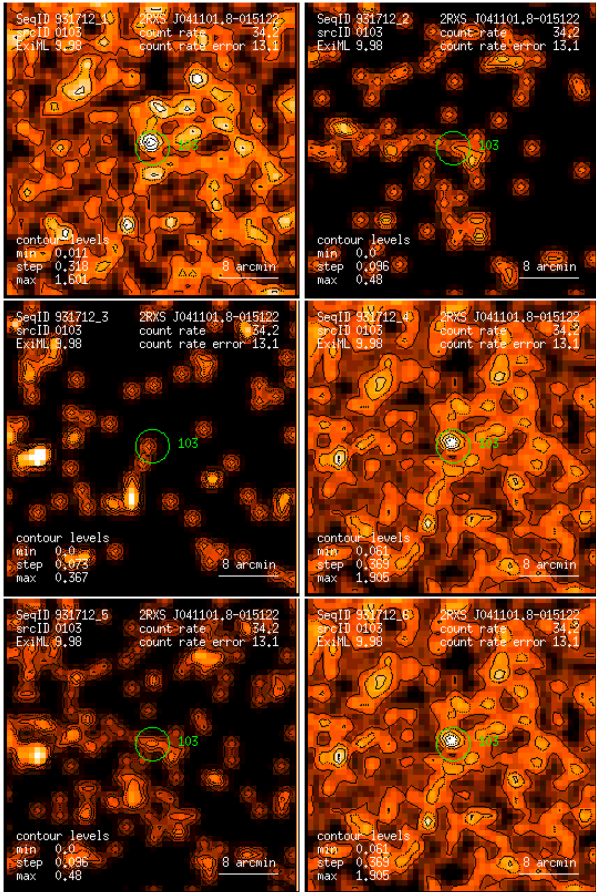
Figure 103: RASS 931712: detection 0103: band rate images, Gaussian filter: (1) PSPC channels 11 – 41, (2) 52 – 90, (3) 91 – 201, (4) 11 – 235, (5) 52 – 201, (6) 11 – 201. Broad band rates in counts/ks. Band rate contour levels in counts/ks/arcmin 2 .
