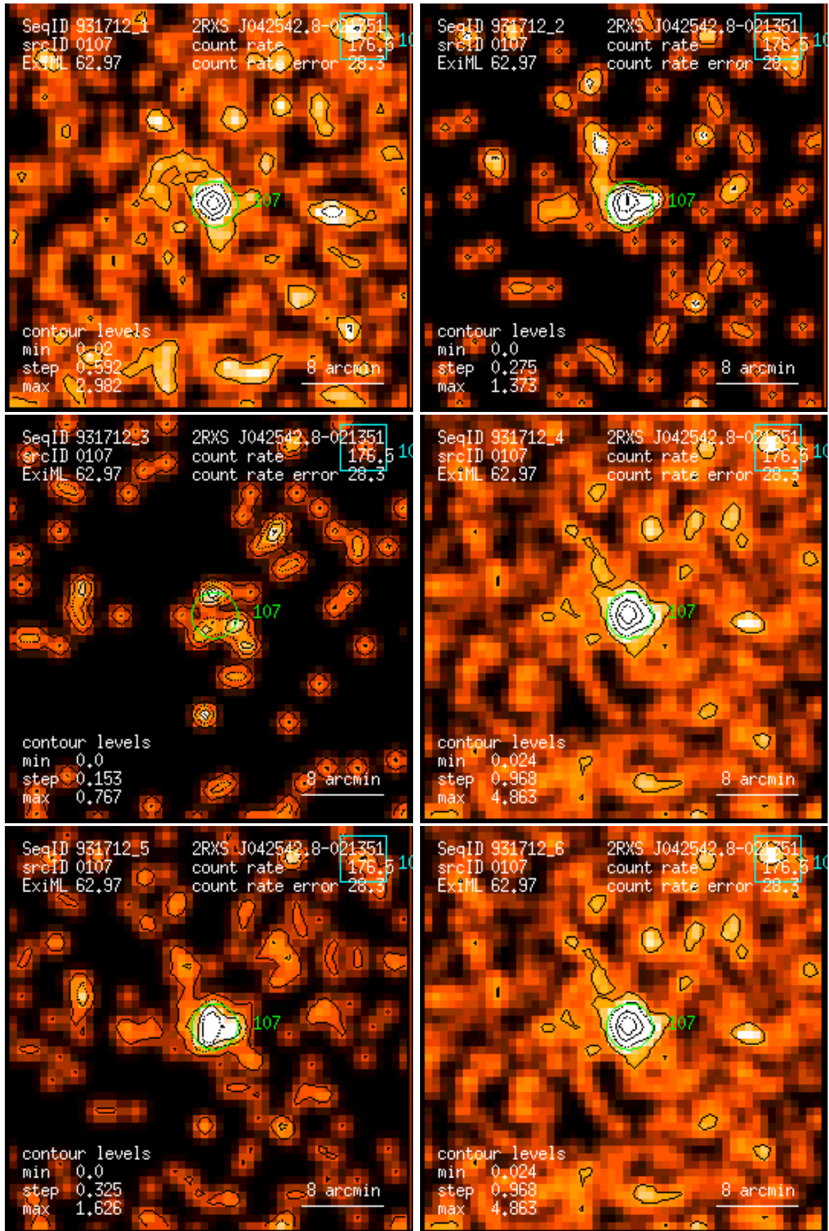
Figure 107: RASS 931712: detection 0107: band rate images, Gaussian filter: (1) PSPC channels 11 – 41, (2) 52 – 90, (3) 91 – 201, (4) 11 – 235, (5) 52 – 201, (6) 11 – 201. Broad band rates in counts/ks. Band rate contour levels in counts/ks/arcmin 2 .
