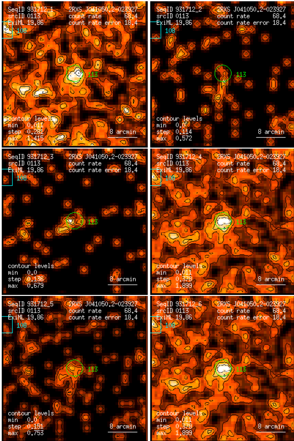
Figure 113: RASS 931712: detection 0113: band rate images, Gaussian filter: (1) PSPC channels 11 – 41, (2) 52 – 90, (3) 91 – 201, (4) 11 – 235, (5) 52 – 201, (6) 11 – 201. Broad band rates in counts/ks. Band rate contour levels in counts/ks/arcmin 2 .
