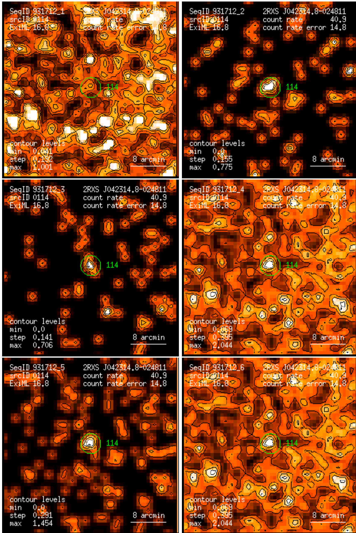
Figure 114: RASS 931712: detection 0114: band rate images, Gaussian filter: (1) PSPC channels 11 – 41, (2) 52 – 90, (3) 91 – 201, (4) 11 – 235, (5) 52 – 201, (6) 11 – 201. Broad band rates in counts/ks. Band rate contour levels in counts/ks/arcmin 2 .
