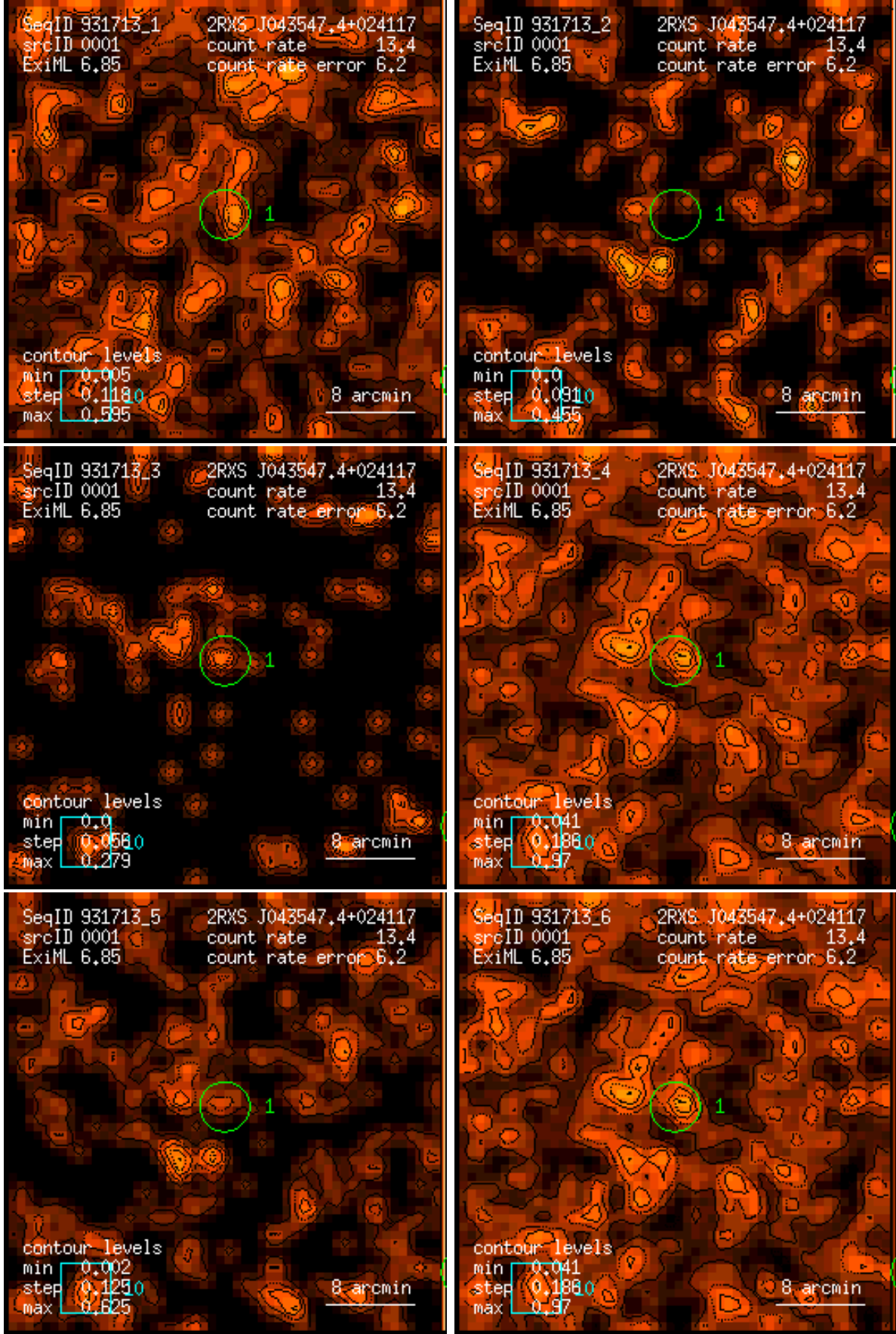
Figure 1: RASS 931713: detection 0001: band rate images, Gaussian filter: (1) PSPC channels 11 – 41, (2) 52 – 90, (3) 91 – 201, (4) 11 – 235, (5) 52 – 201, (6) 11 – 201. Broad band rates in counts/ks. Band rate contour levels in counts/ks/arcmin 2 .
