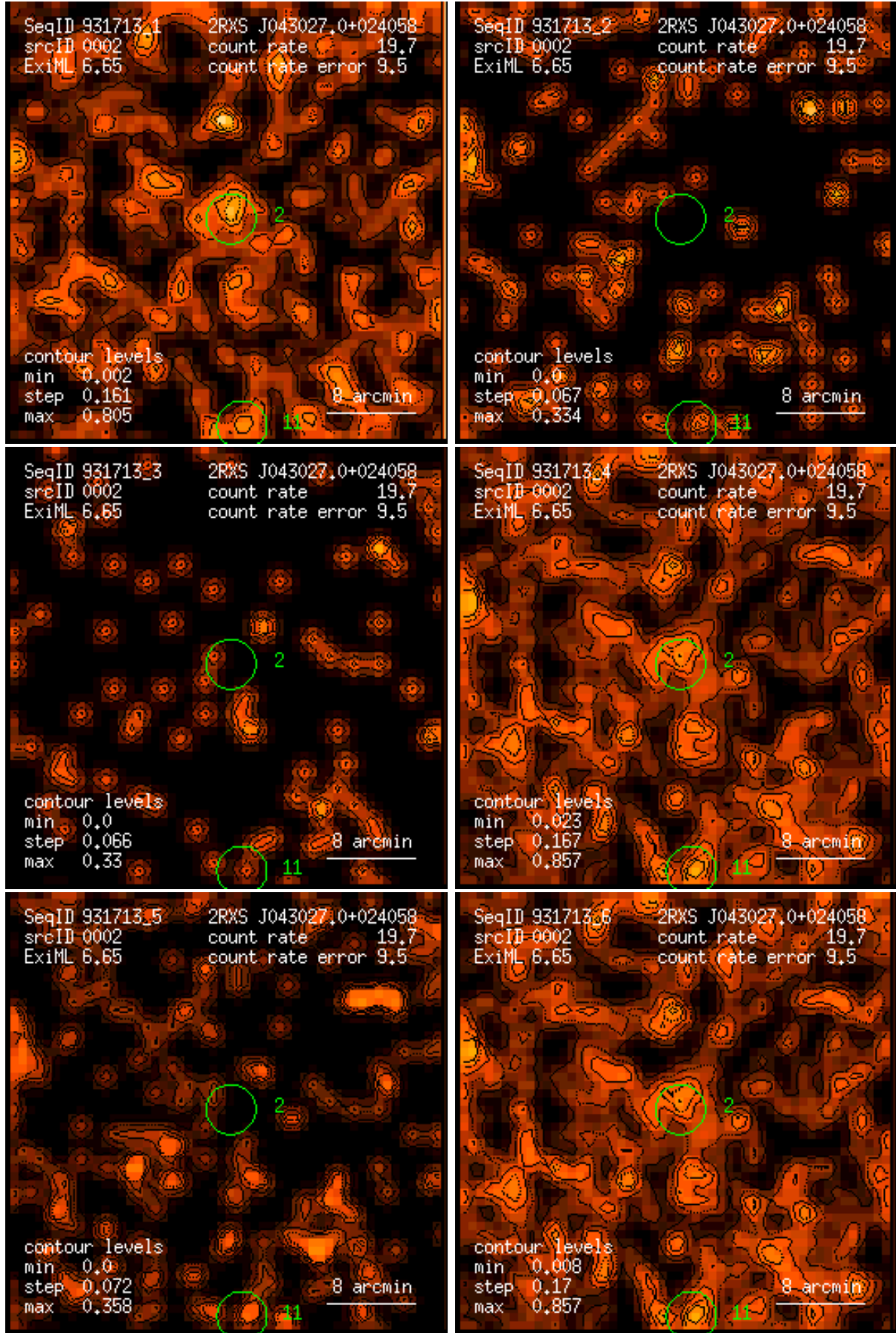
Figure 2: RASS 931713: detection 0002: band rate images, Gaussian filter: (1) PSPC channels 11 – 41, (2) 52 – 90, (3) 91 – 201, (4) 11 – 235, (5) 52 – 201, (6) 11 – 201. Broad band rates in counts/ks. Band rate contour levels in counts/ks/arcmin 2 .
