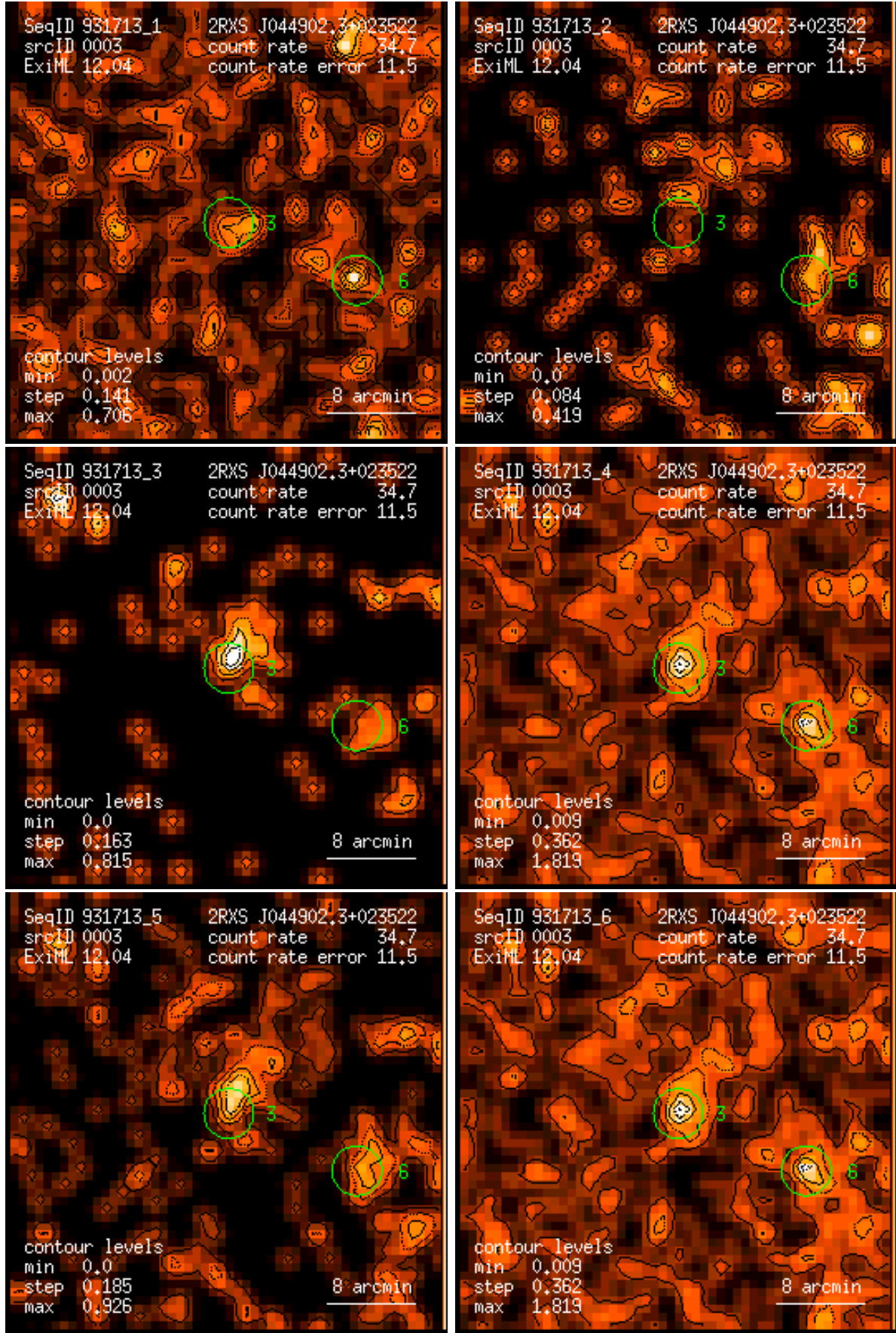
Figure 3: RASS 931713: detection 0003: band rate images, Gaussian filter: (1) PSPC channels 11 – 41, (2) 52 – 90, (3) 91 – 201, (4) 11 – 235, (5) 52 – 201, (6) 11 – 201. Broad band rates in counts/ks. Band rate contour levels in counts/ks/arcmin 2 .
