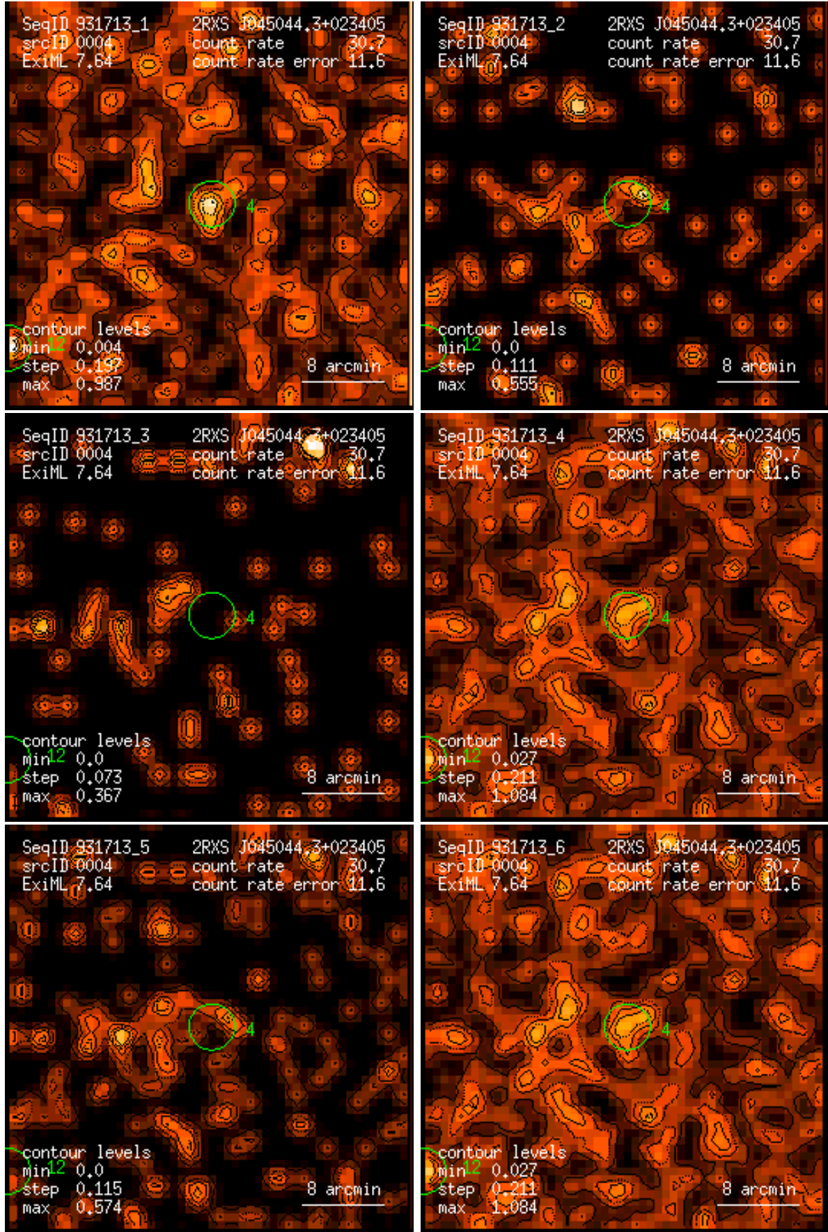
Figure 4: RASS 931713: detection 0004: band rate images, Gaussian filter: (1) PSPC channels 11 – 41, (2) 52 – 90, (3) 91 – 201, (4) 11 – 235, (5) 52 – 201, (6) 11 – 201. Broad band rates in counts/ks. Band rate contour levels in counts/ks/arcmin 2 .
