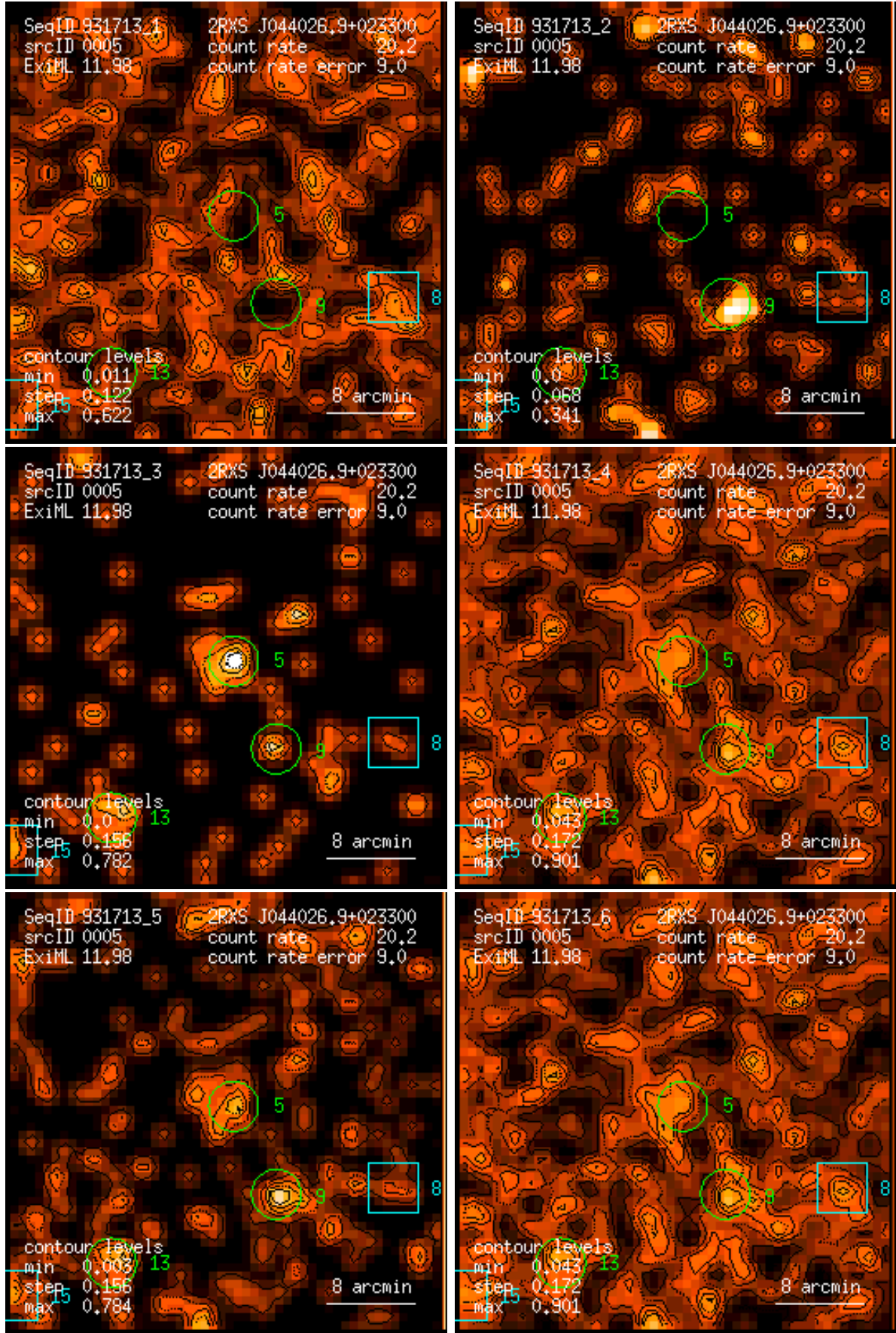
Figure 5: RASS 931713: detection 0005: band rate images, Gaussian filter: (1) PSPC channels 11 – 41, (2) 52 – 90, (3) 91 – 201, (4) 11 – 235, (5) 52 – 201, (6) 11 – 201. Broad band rates in counts/ks. Band rate contour levels in counts/ks/arcmin 2 .
