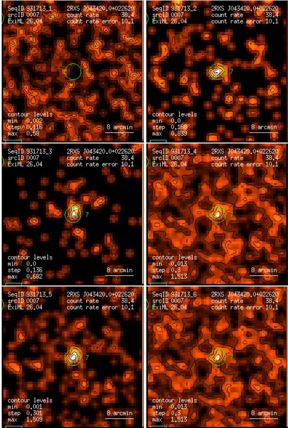
Figure 7: RASS 931713: detection 0007: band rate images, Gaussian filter: (1) PSPC channels 11 – 41, (2) 52 – 90, (3) 91 – 201, (4) 11 – 235, (5) 52 – 201, (6) 11 – 201. Broad band rates in counts/ks. Band rate contour levels in counts/ks/arcmin 2 .
