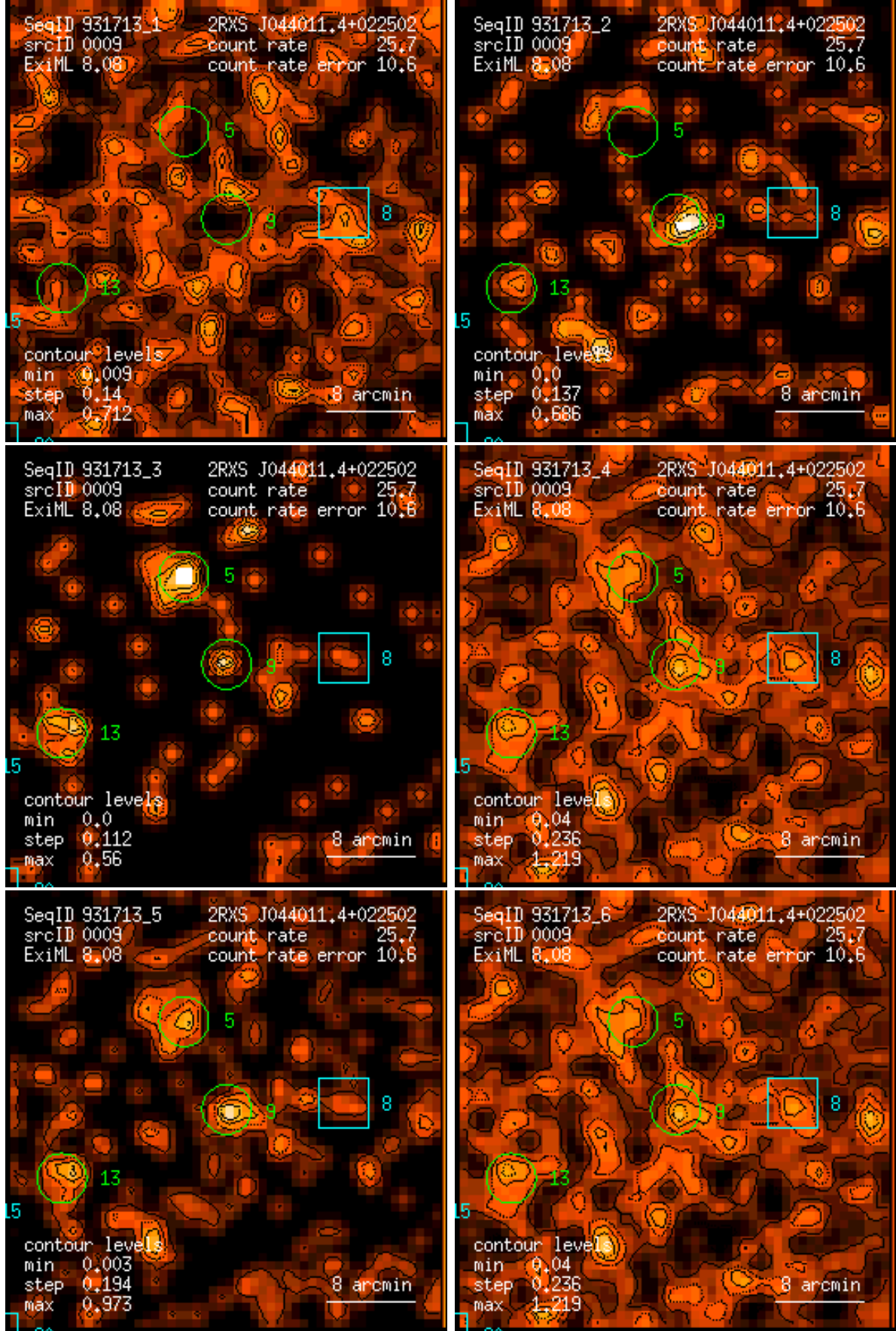
Figure 9: RASS 931713: detection 0009: band rate images, Gaussian filter: (1) PSPC channels 11 – 41, (2) 52 – 90, (3) 91 – 201, (4) 11 – 235, (5) 52 – 201, (6) 11 – 201. Broad band rates in counts/ks. Band rate contour levels in counts/ks/arcmin 2 .
