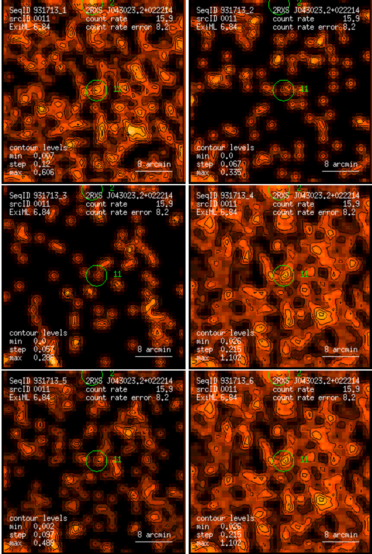
Figure 11: RASS 931713: detection 0011: band rate images, Gaussian filter: (1) PSPC channels 11 – 41, (2) 52 – 90, (3) 91 – 201, (4) 11 – 235, (5) 52 – 201, (6) 11 – 201. Broad band rates in counts/ks. Band rate contour levels in counts/ks/arcmin 2 .
