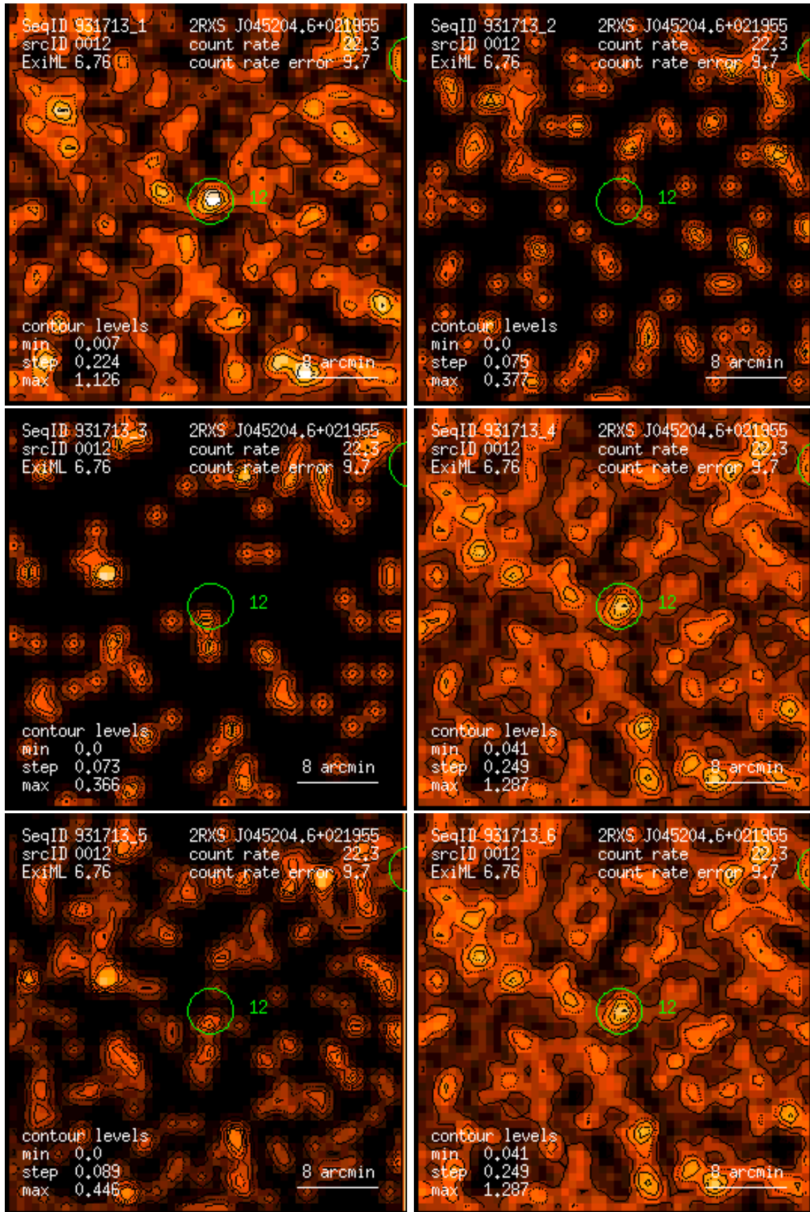
Figure 12: RASS 931713: detection 0012: band rate images, Gaussian filter: (1) PSPC channels 11 – 41, (2) 52 – 90, (3) 91 – 201, (4) 11 – 235, (5) 52 – 201, (6) 11 – 201. Broad band rates in counts/ks. Band rate contour levels in counts/ks/arcmin 2 .
