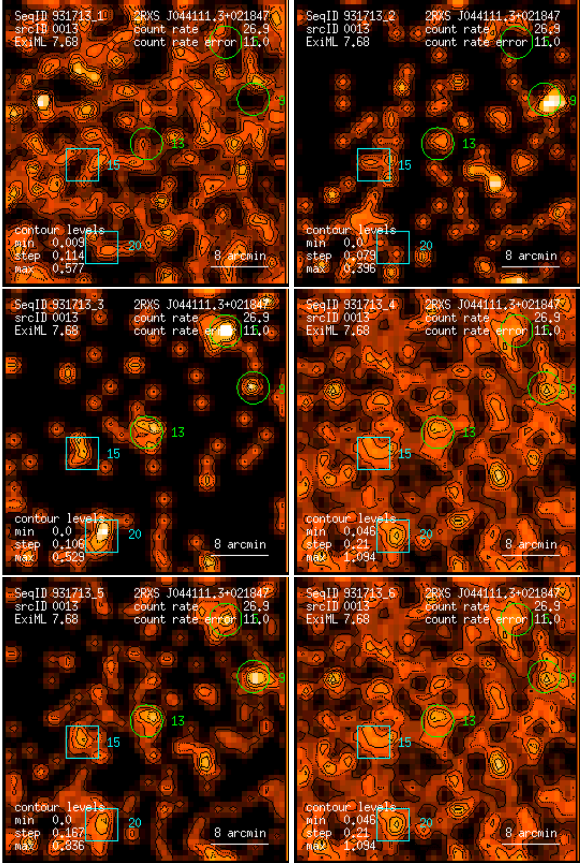
Figure 13: RASS 931713: detection 0013: band rate images, Gaussian filter: (1) PSPC channels 11 – 41, (2) 52 – 90, (3) 91 – 201, (4) 11 – 235, (5) 52 – 201, (6) 11 – 201. Broad band rates in counts/ks. Band rate contour levels in counts/ks/arcmin 2 .
