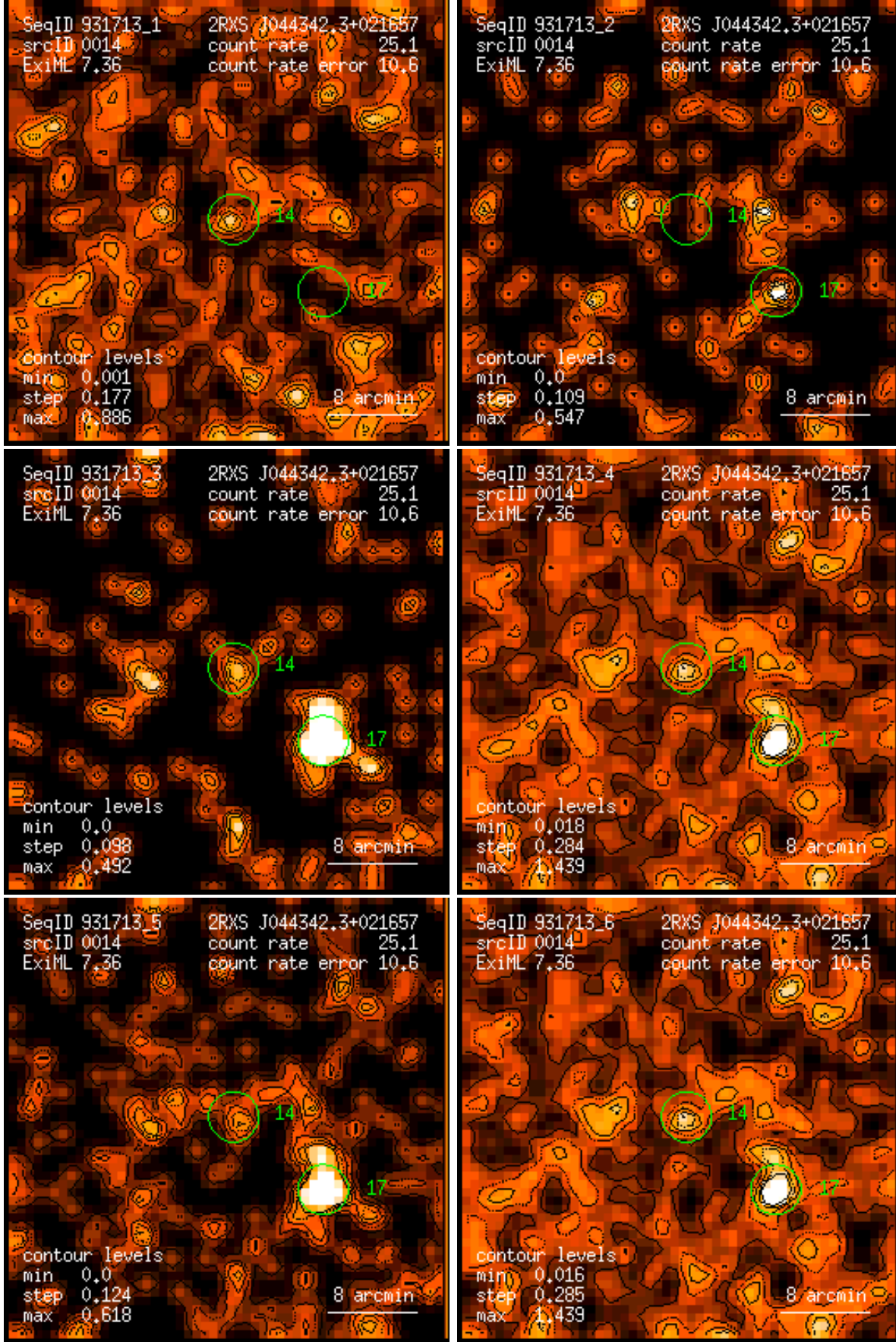
Figure 14: RASS 931713: detection 0014: band rate images, Gaussian filter: (1) PSPC channels 11 – 41, (2) 52 – 90, (3) 91 – 201, (4) 11 – 235, (5) 52 – 201, (6) 11 – 201. Broad band rates in counts/ks. Band rate contour levels in counts/ks/arcmin 2 .
