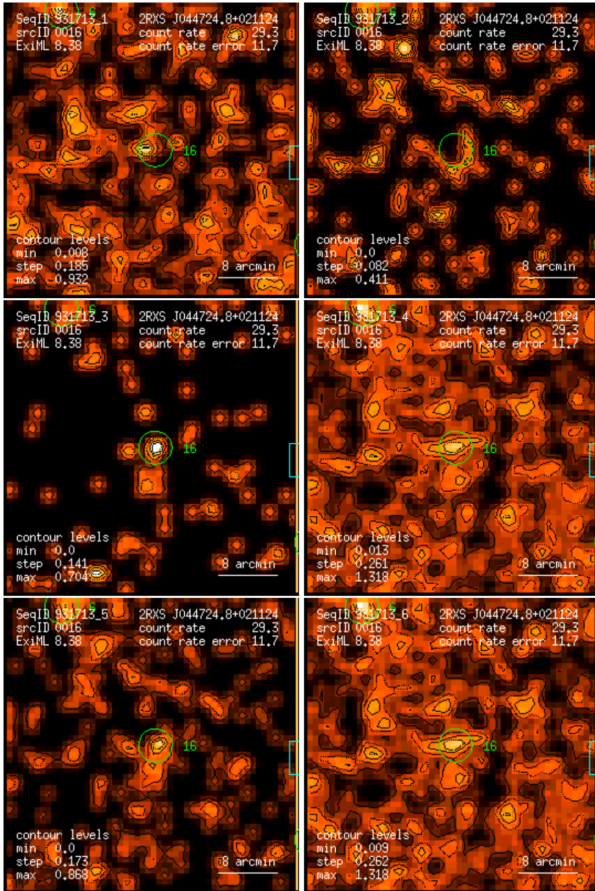
Figure 16: RASS 931713: detection 0016: band rate images, Gaussian filter: (1) PSPC channels 11 – 41, (2) 52 – 90, (3) 91 – 201, (4) 11 – 235, (5) 52 – 201, (6) 11 – 201. Broad band rates in counts/ks. Band rate contour levels in counts/ks/arcmin 2 .
