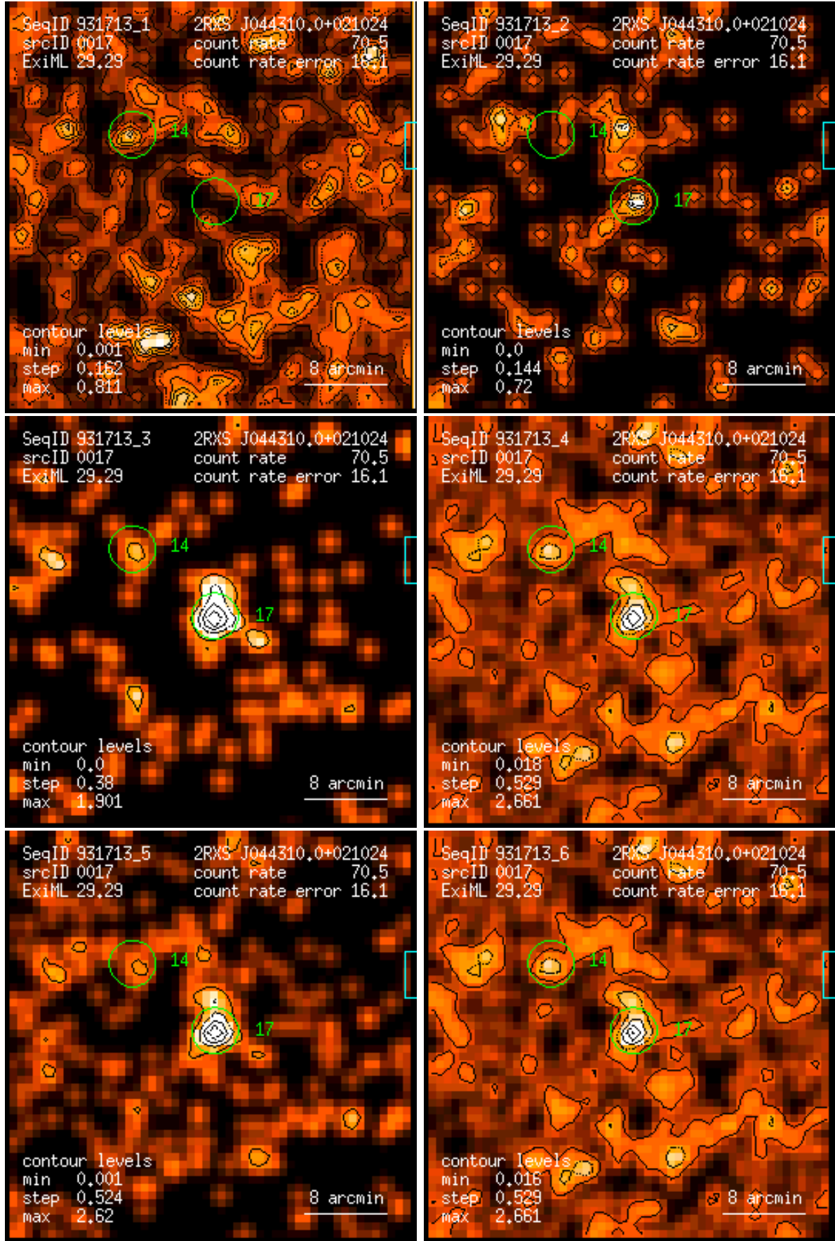
Figure 17: RASS 931713: detection 0017: band rate images, Gaussian filter: (1) PSPC channels 11 – 41, (2) 52 – 90, (3) 91 – 201, (4) 11 – 235, (5) 52 – 201, (6) 11 – 201. Broad band rates in counts/ks. Band rate contour levels in counts/ks/arcmin 2 .
