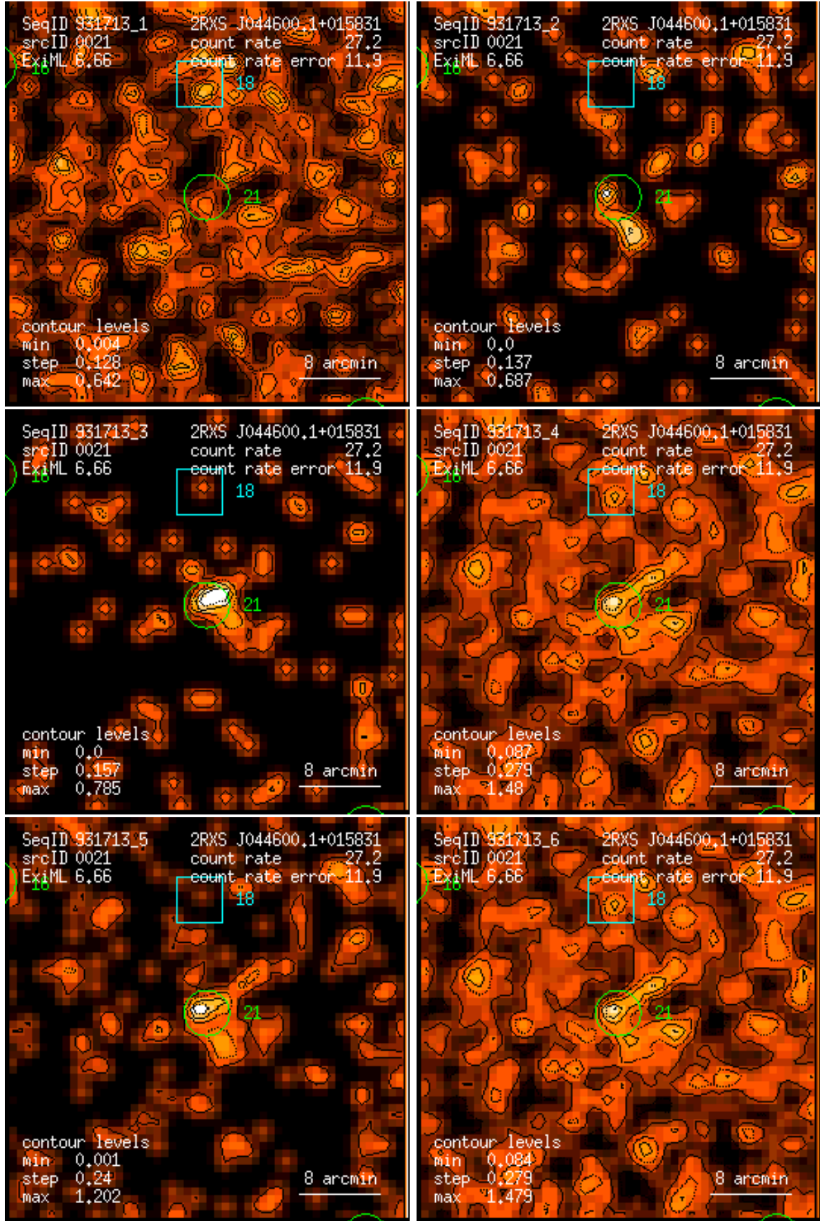
Figure 21: RASS 931713: detection 0021: band rate images, Gaussian filter: (1) PSPC channels 11 – 41, (2) 52 – 90, (3) 91 – 201, (4) 11 – 235, (5) 52 – 201, (6) 11 – 201. Broad band rates in counts/ks. Band rate contour levels in counts/ks/arcmin 2 .
