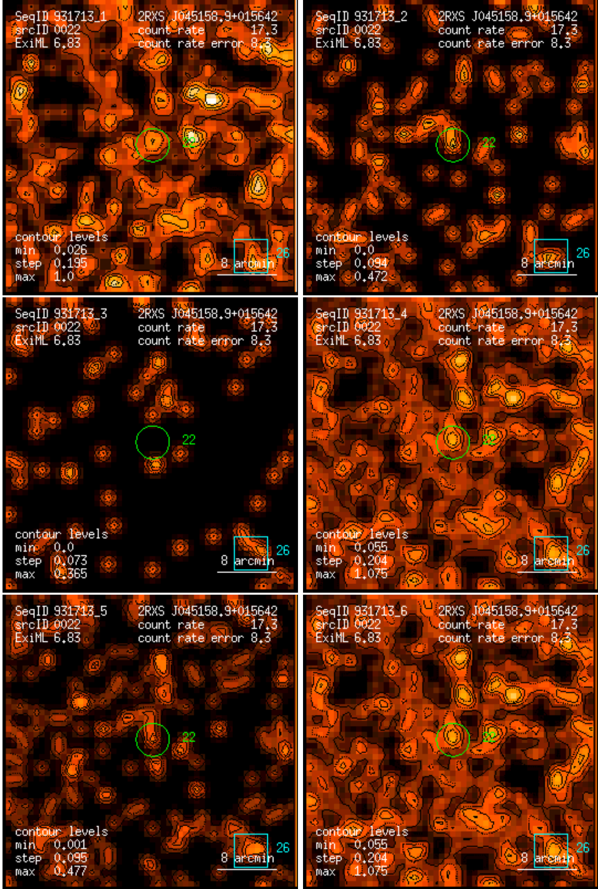
Figure 22: RASS 931713: detection 0022: band rate images, Gaussian filter: (1) PSPC channels 11 – 41, (2) 52 – 90, (3) 91 – 201, (4) 11 – 235, (5) 52 – 201, (6) 11 – 201. Broad band rates in counts/ks. Band rate contour levels in counts/ks/arcmin 2 .
