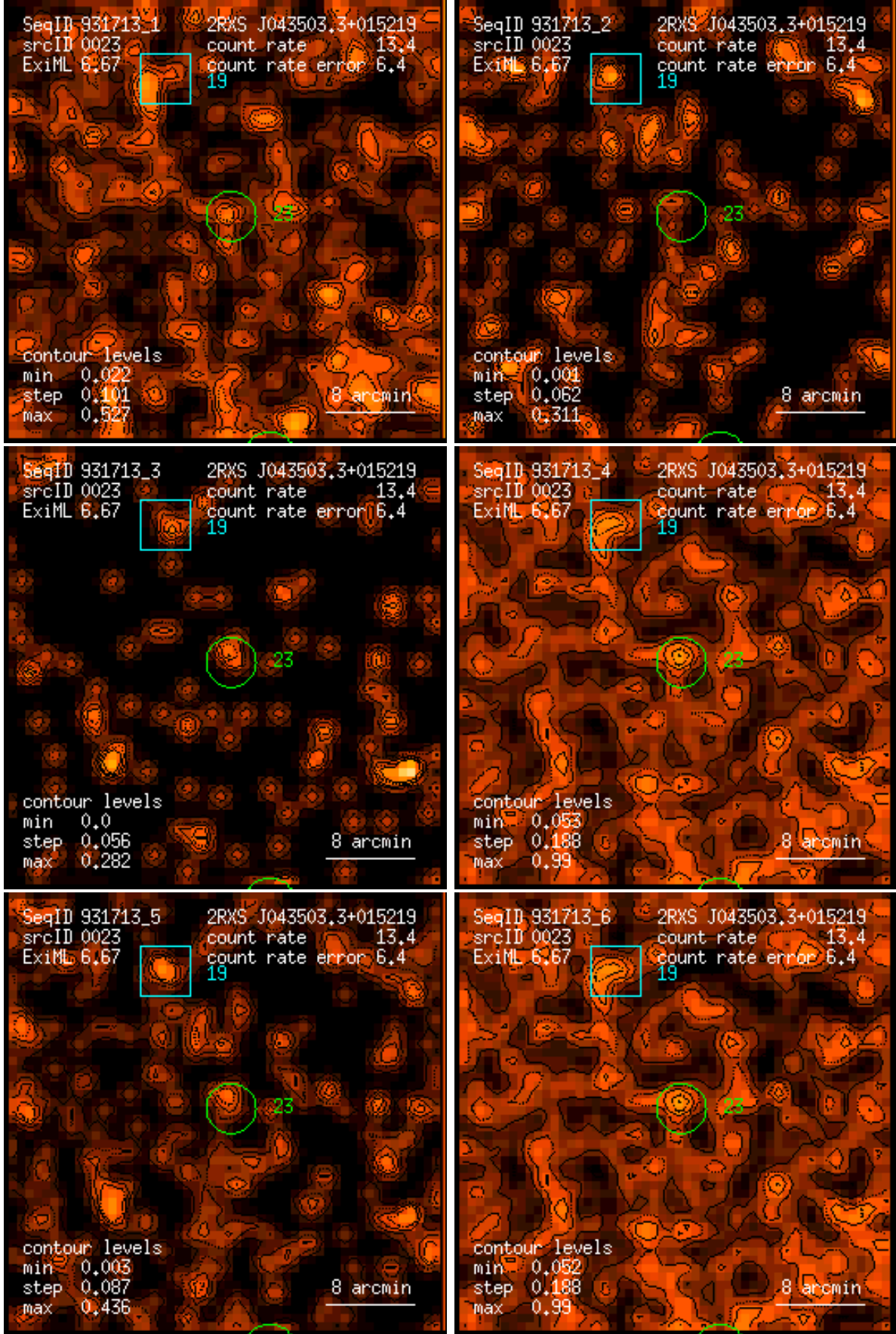
Figure 23: RASS 931713: detection 0023: band rate images, Gaussian filter: (1) PSPC channels 11 – 41, (2) 52 – 90, (3) 91 – 201, (4) 11 – 235, (5) 52 – 201, (6) 11 – 201. Broad band rates in counts/ks. Band rate contour levels in counts/ks/arcmin 2 .
