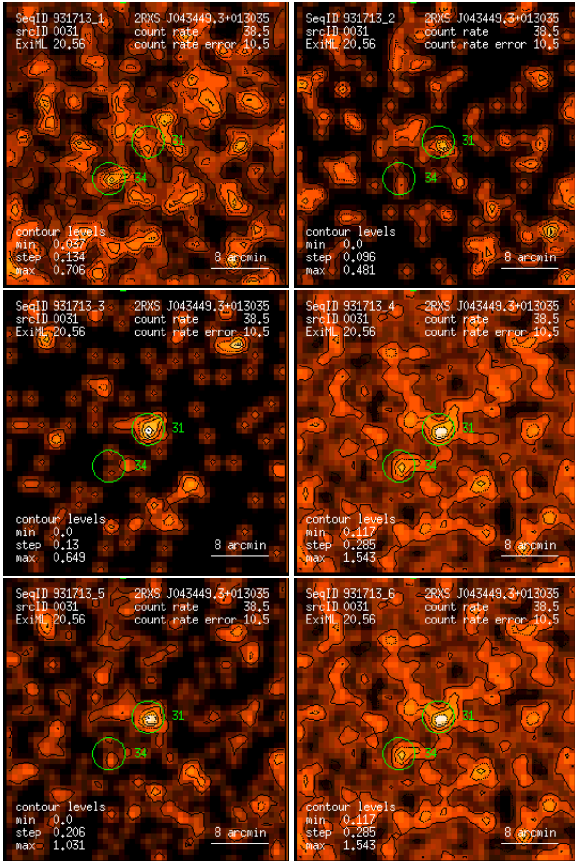
Figure 31: RASS 931713: detection 0031: band rate images, Gaussian filter: (1) PSPC channels 11 – 41, (2) 52 – 90, (3) 91 – 201, (4) 11 – 235, (5) 52 – 201, (6) 11 – 201. Broad band rates in counts/ks. Band rate contour levels in counts/ks/arcmin 2 .
