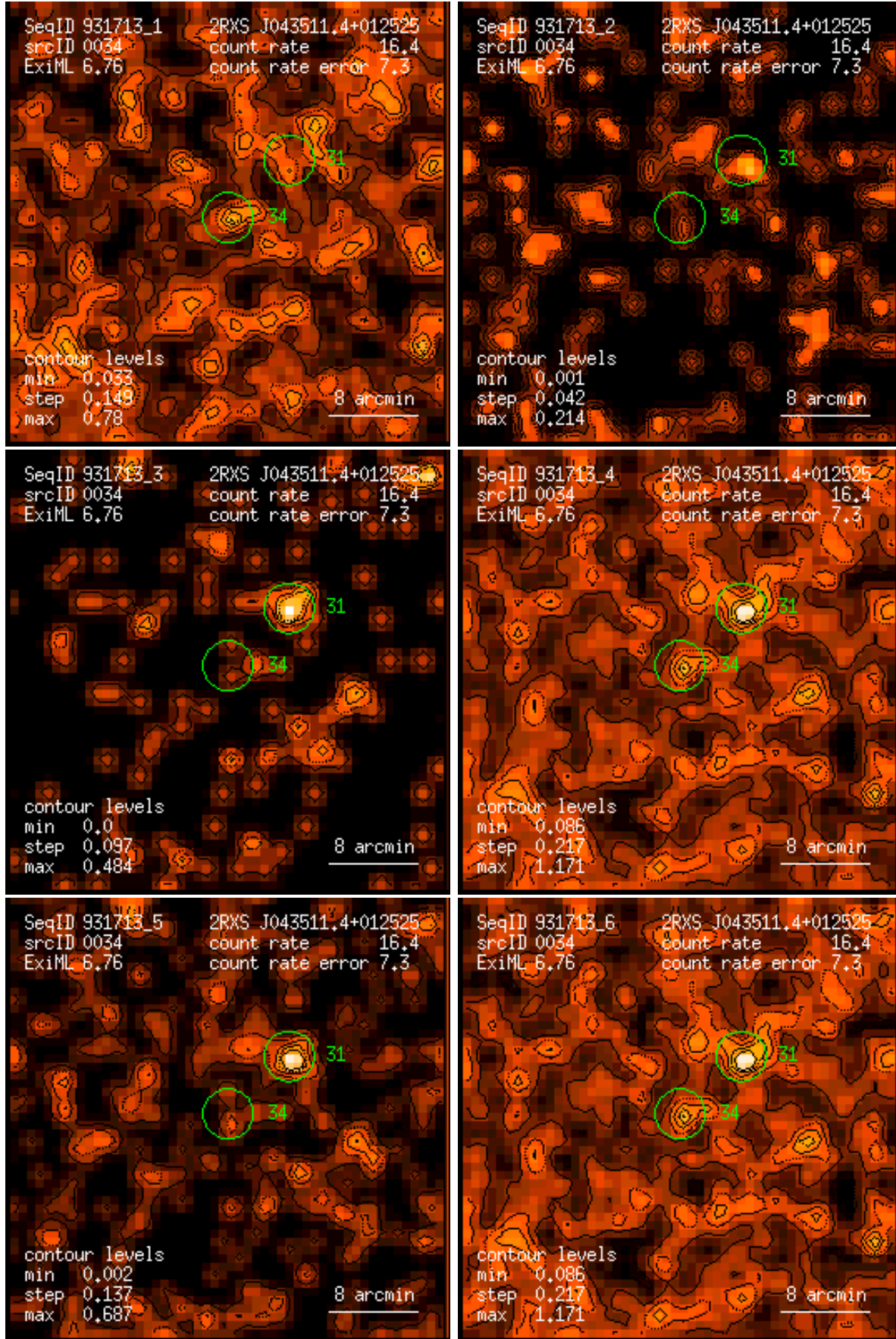
Figure 34: RASS 931713: detection 0034: band rate images, Gaussian filter: (1) PSPC channels 11 – 41, (2) 52 – 90, (3) 91 – 201, (4) 11 – 235, (5) 52 – 201, (6) 11 – 201. Broad band rates in counts/ks. Band rate contour levels in counts/ks/arcmin 2 .
