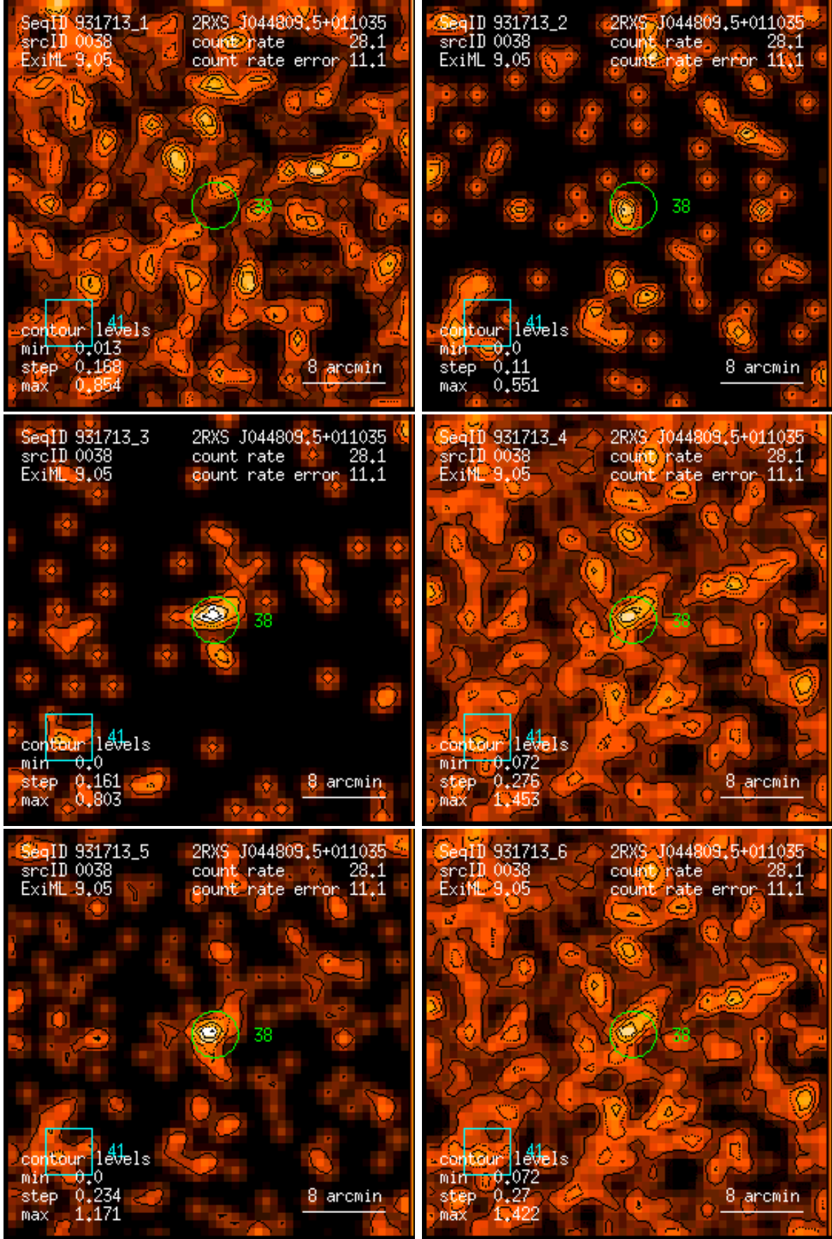
Figure 38: RASS 931713: detection 0038: band rate images, Gaussian filter: (1) PSPC channels 11 – 41, (2) 52 – 90, (3) 91 – 201, (4) 11 – 235, (5) 52 – 201, (6) 11 – 201. Broad band rates in counts/ks. Band rate contour levels in counts/ks/arcmin 2 .
