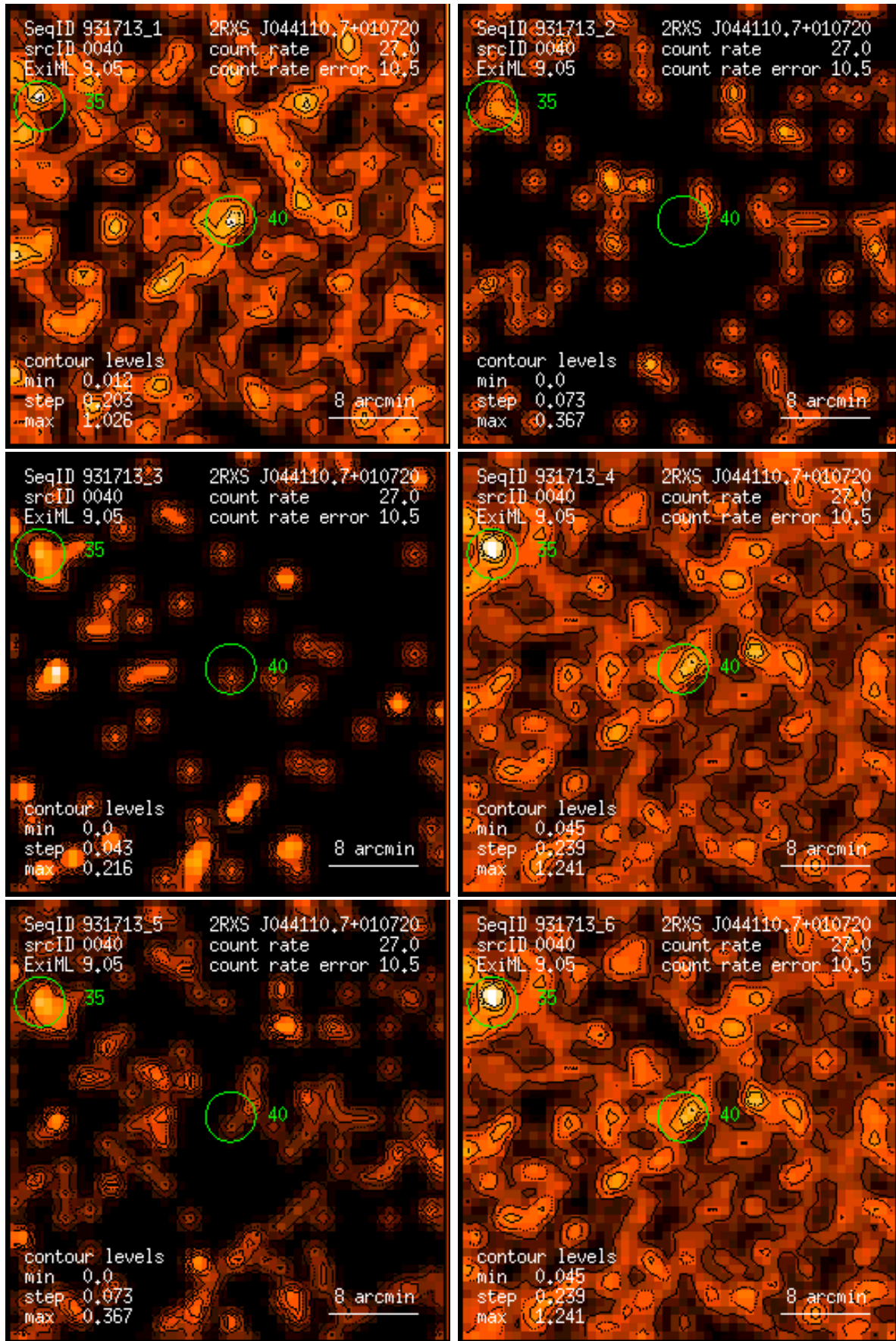
Figure 40: RASS 931713: detection 0040: band rate images, Gaussian filter: (1) PSPC channels 11 – 41, (2) 52 – 90, (3) 91 – 201, (4) 11 – 235, (5) 52 – 201, (6) 11 – 201. Broad band rates in counts/ks. Band rate contour levels in counts/ks/arcmin 2 .
