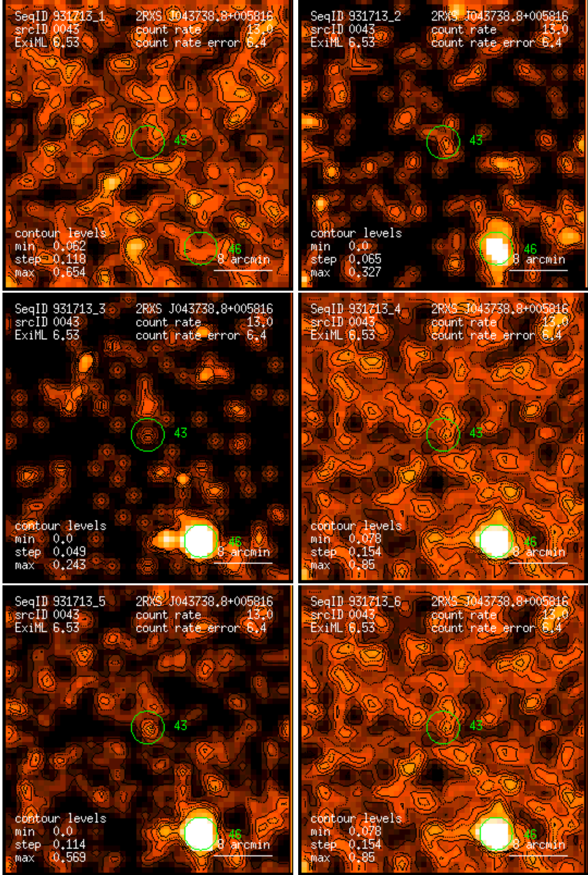
Figure 43: RASS 931713: detection 0043: band rate images, Gaussian filter: (1) PSPC channels 11 – 41, (2) 52 – 90, (3) 91 – 201, (4) 11 – 235, (5) 52 – 201, (6) 11 – 201. Broad band rates in counts/ks. Band rate contour levels in counts/ks/arcmin 2 .
