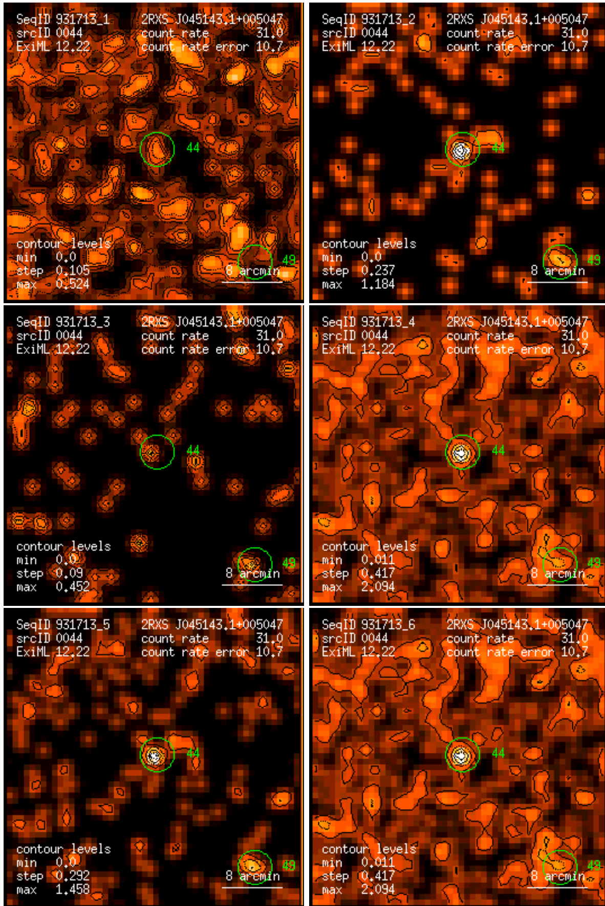
Figure 44: RASS 931713: detection 0044: band rate images, Gaussian filter: (1) PSPC channels 11 – 41, (2) 52 – 90, (3) 91 – 201, (4) 11 – 235, (5) 52 – 201, (6) 11 – 201. Broad band rates in counts/ks. Band rate contour levels in counts/ks/arcmin 2 .
