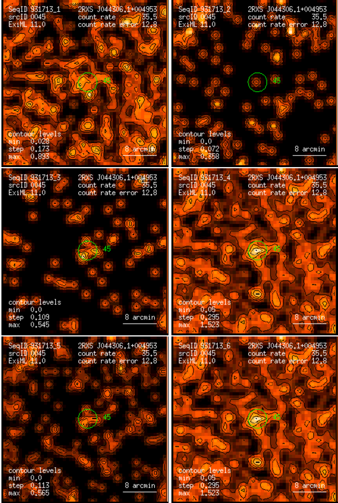
Figure 45: RASS 931713: detection 0045: band rate images, Gaussian filter: (1) PSPC channels 11 – 41, (2) 52 – 90, (3) 91 – 201, (4) 11 – 235, (5) 52 – 201, (6) 11 – 201. Broad band rates in counts/ks. Band rate contour levels in counts/ks/arcmin 2 .
