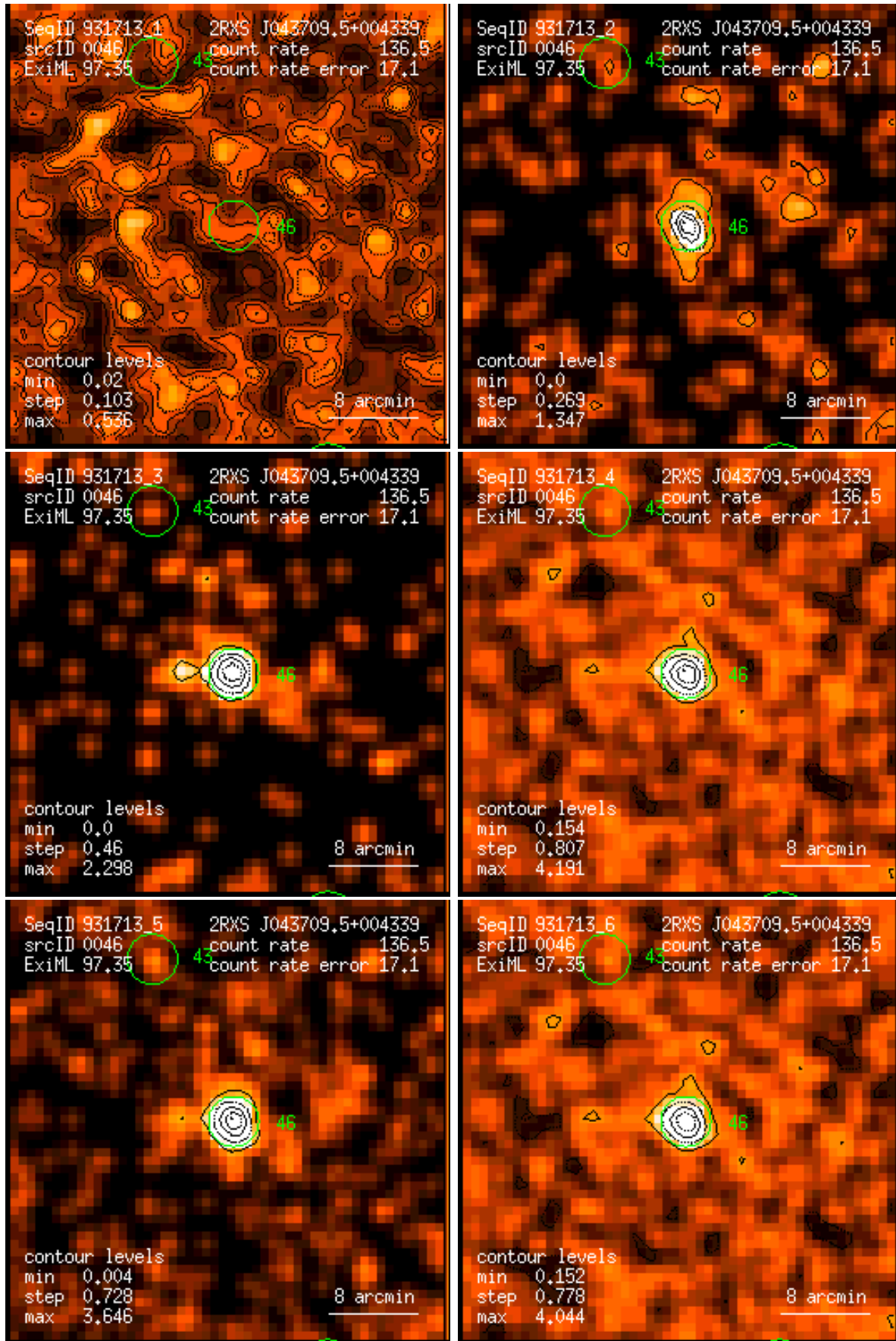
Figure 46: RASS 931713: detection 0046: band rate images, Gaussian filter: (1) PSPC channels 11 – 41, (2) 52 – 90, (3) 91 – 201, (4) 11 – 235, (5) 52 – 201, (6) 11 – 201. Broad band rates in counts/ks. Band rate contour levels in counts/ks/arcmin 2 .
