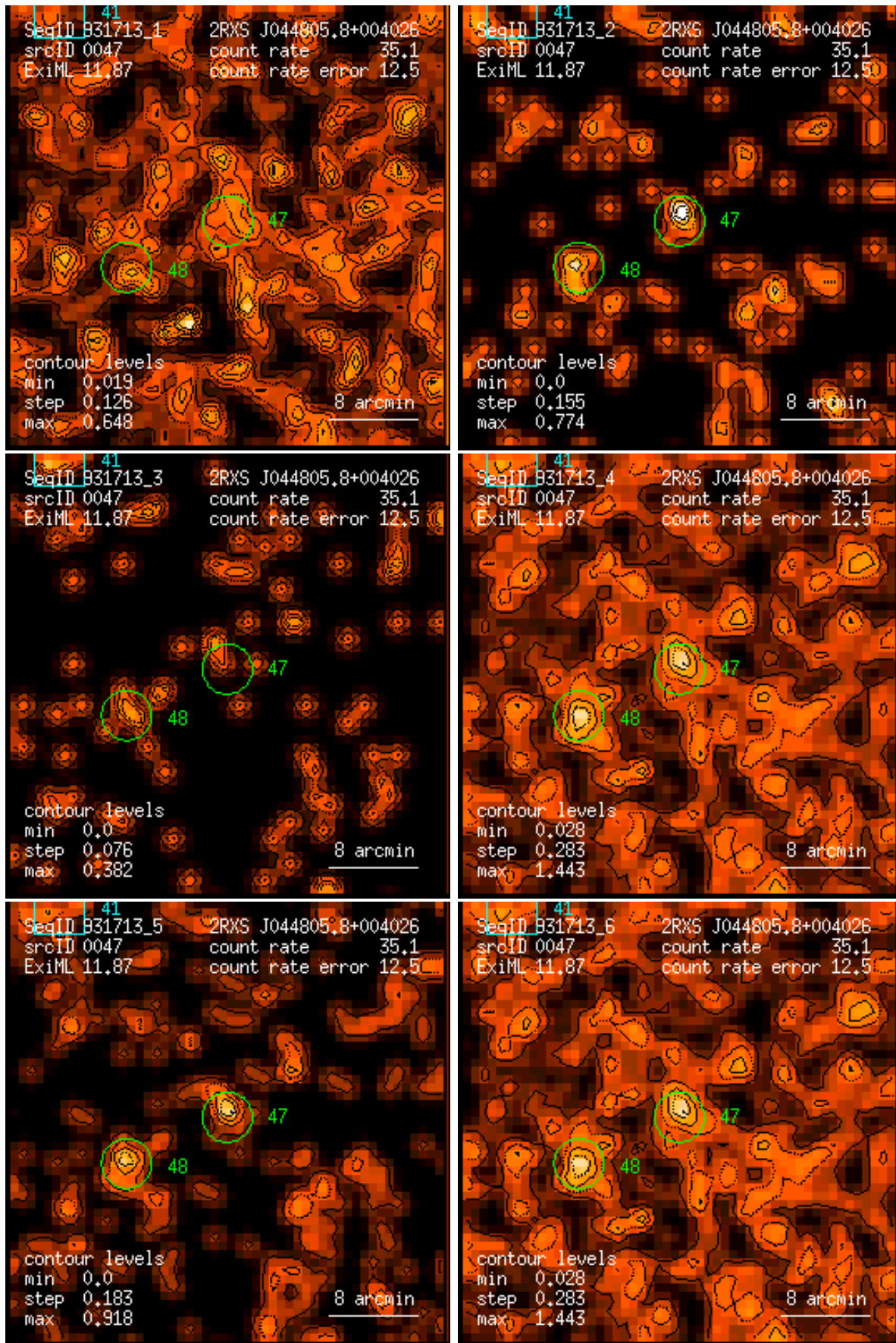
Figure 47: RASS 931713: detection 0047: band rate images, Gaussian filter: (1) PSPC channels 11 – 41, (2) 52 – 90, (3) 91 – 201, (4) 11 – 235, (5) 52 – 201, (6) 11 – 201. Broad band rates in counts/ks. Band rate contour levels in counts/ks/arcmin 2 .
