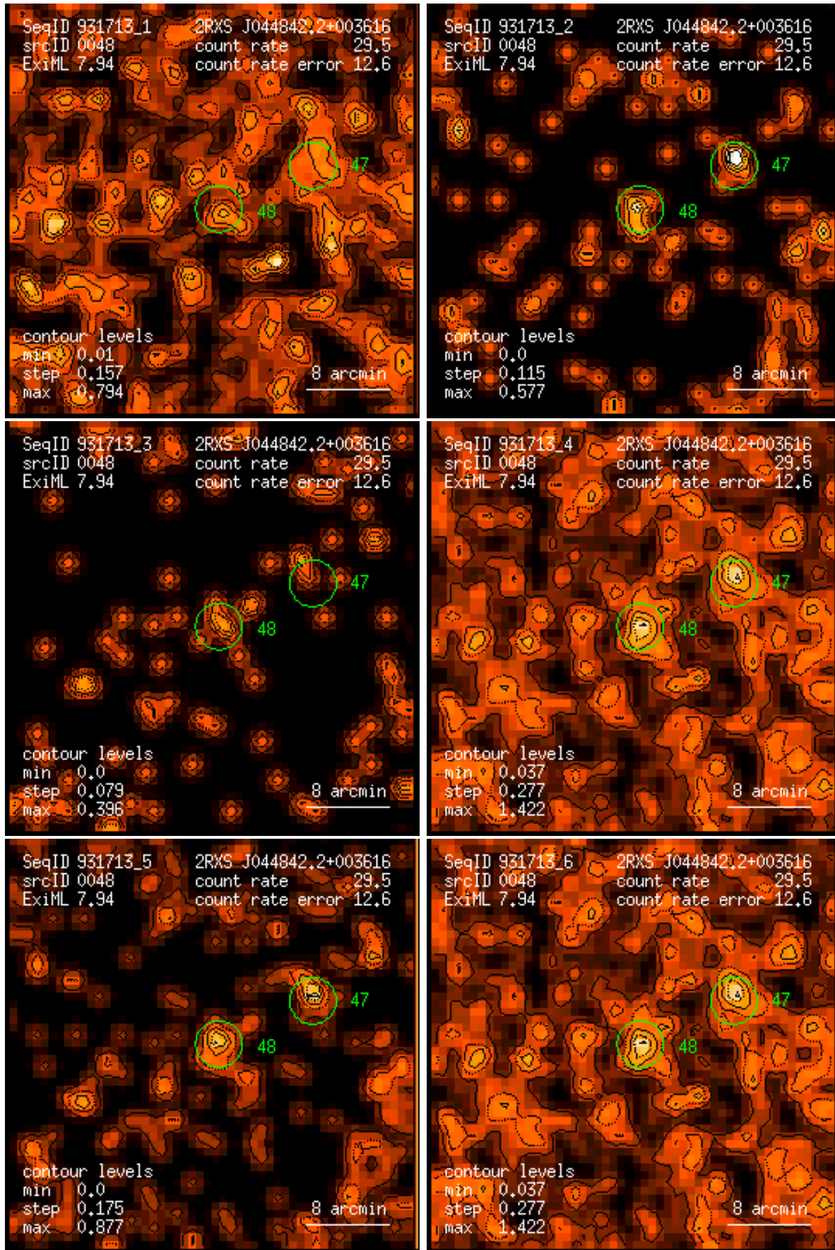
Figure 48: RASS 931713: detection 0048: band rate images, Gaussian filter: (1) PSPC channels 11 – 41, (2) 52 – 90, (3) 91 – 201, (4) 11 – 235, (5) 52 – 201, (6) 11 – 201. Broad band rates in counts/ks. Band rate contour levels in counts/ks/arcmin 2 .
