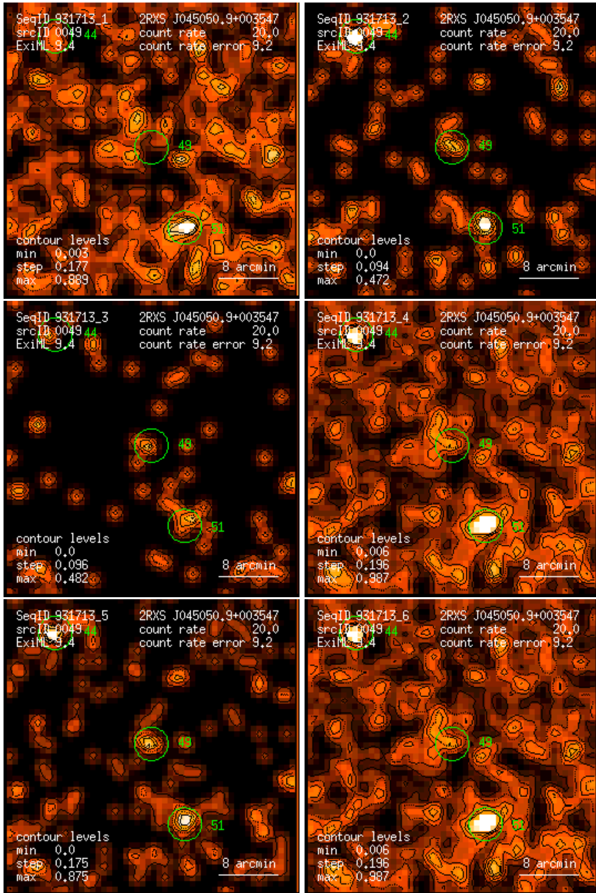
Figure 49: RASS 931713: detection 0049: band rate images, Gaussian filter: (1) PSPC channels 11 – 41, (2) 52 – 90, (3) 91 – 201, (4) 11 – 235, (5) 52 – 201, (6) 11 – 201. Broad band rates in counts/ks. Band rate contour levels in counts/ks/arcmin 2 .
