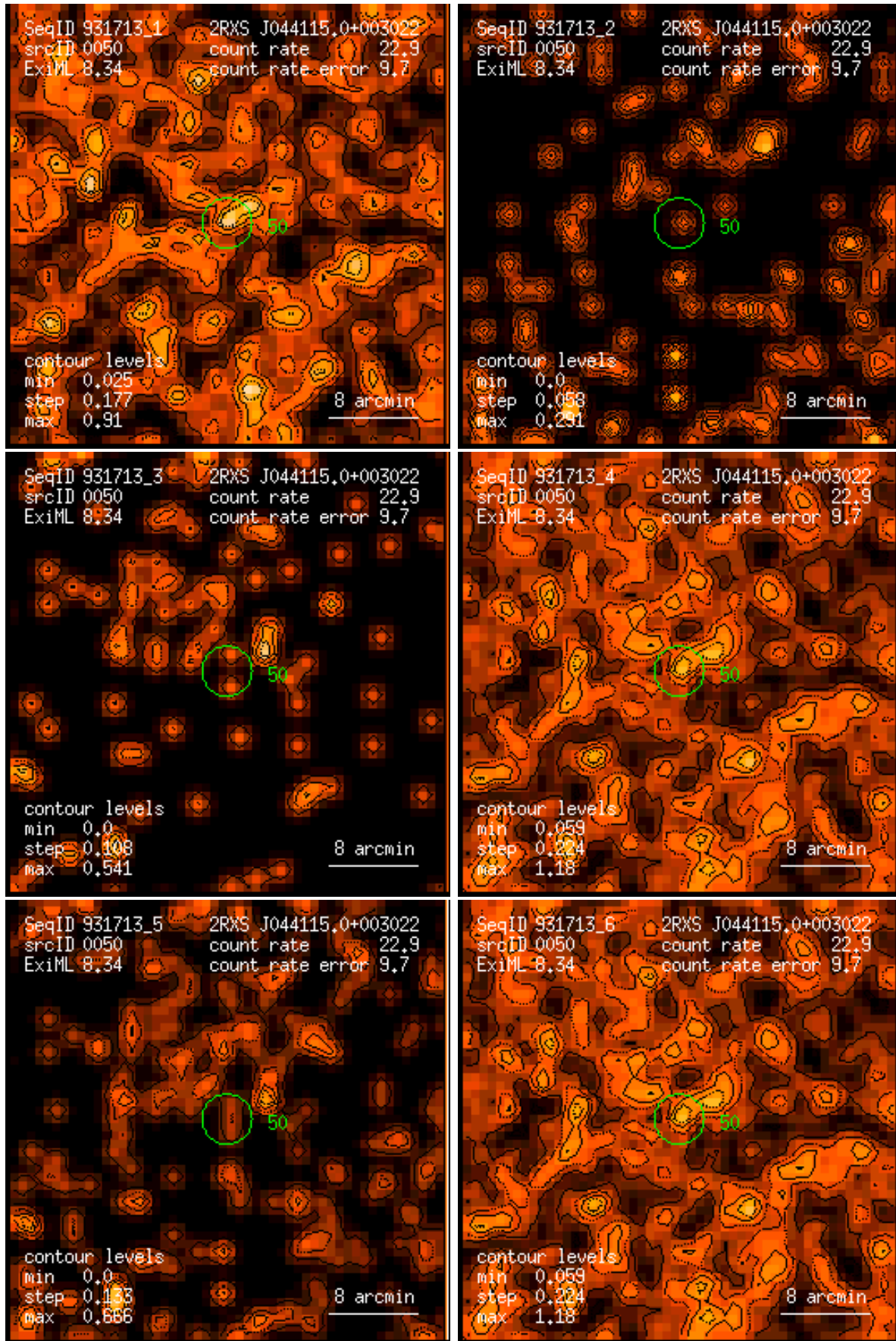
Figure 50: RASS 931713: detection 0050: band rate images, Gaussian filter: (1) PSPC channels 11 – 41, (2) 52 – 90, (3) 91 – 201, (4) 11 – 235, (5) 52 – 201, (6) 11 – 201. Broad band rates in counts/ks. Band rate contour levels in counts/ks/arcmin 2 .
