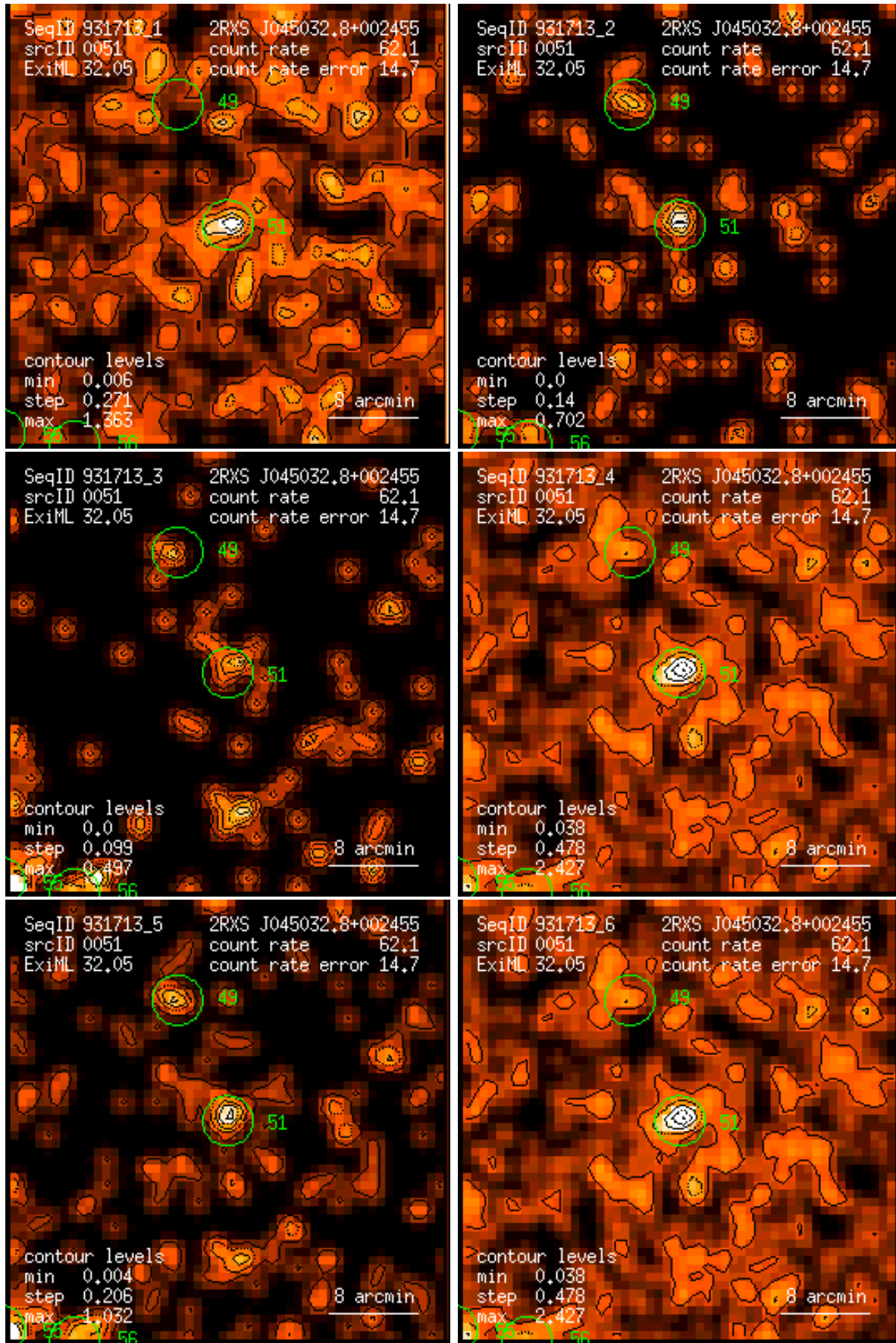
Figure 51: RASS 931713: detection 0051: band rate images, Gaussian filter: (1) PSPC channels 11 – 41, (2) 52 – 90, (3) 91 – 201, (4) 11 – 235, (5) 52 – 201, (6) 11 – 201. Broad band rates in counts/ks. Band rate contour levels in counts/ks/arcmin 2 .
