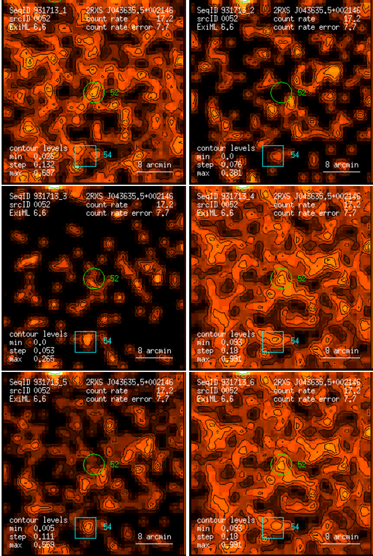
Figure 52: RASS 931713: detection 0052: band rate images, Gaussian filter: (1) PSPC channels 11 – 41, (2) 52 – 90, (3) 91 – 201, (4) 11 – 235, (5) 52 – 201, (6) 11 – 201. Broad band rates in counts/ks. Band rate contour levels in counts/ks/arcmin 2 .
