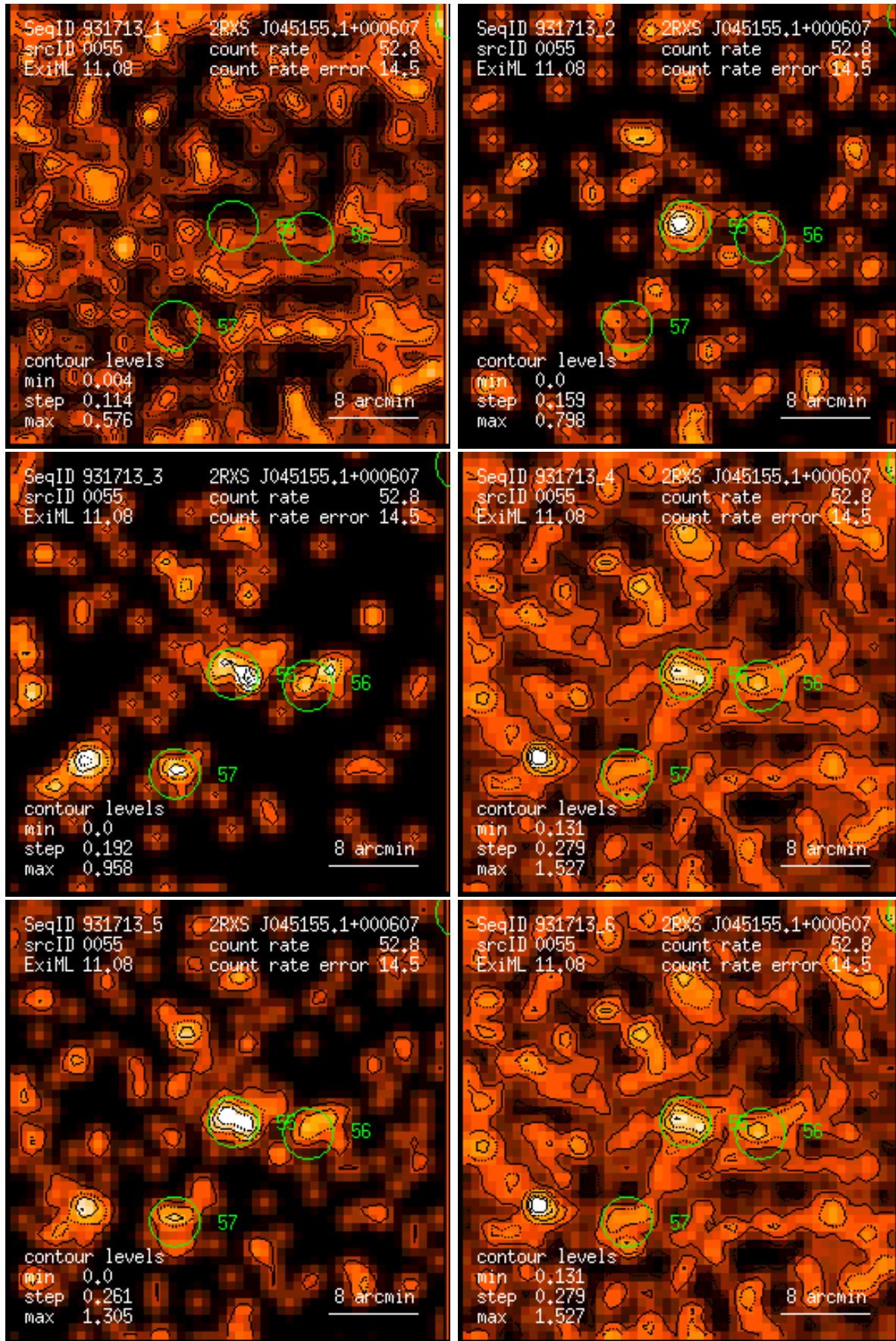
Figure 55: RASS 931713: detection 0055: band rate images, Gaussian filter: (1) PSPC channels 11 – 41, (2) 52 – 90, (3) 91 – 201, (4) 11 – 235, (5) 52 – 201, (6) 11 – 201. Broad band rates in counts/ks. Band rate contour levels in counts/ks/arcmin 2 .
