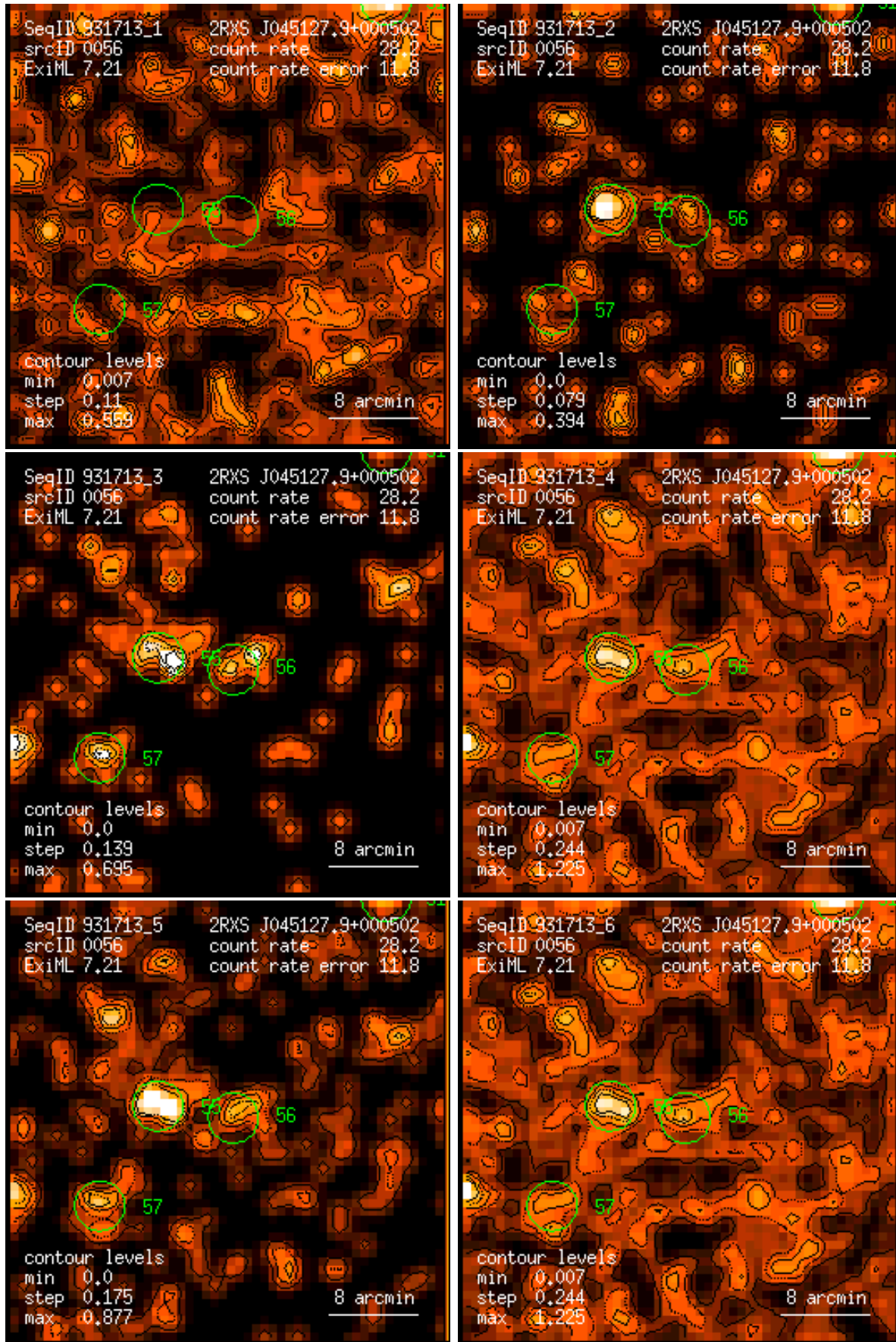
Figure 56: RASS 931713: detection 0056: band rate images, Gaussian filter: (1) PSPC channels 11 – 41, (2) 52 – 90, (3) 91 – 201, (4) 11 – 235, (5) 52 – 201, (6) 11 – 201. Broad band rates in counts/ks. Band rate contour levels in counts/ks/arcmin 2 .
