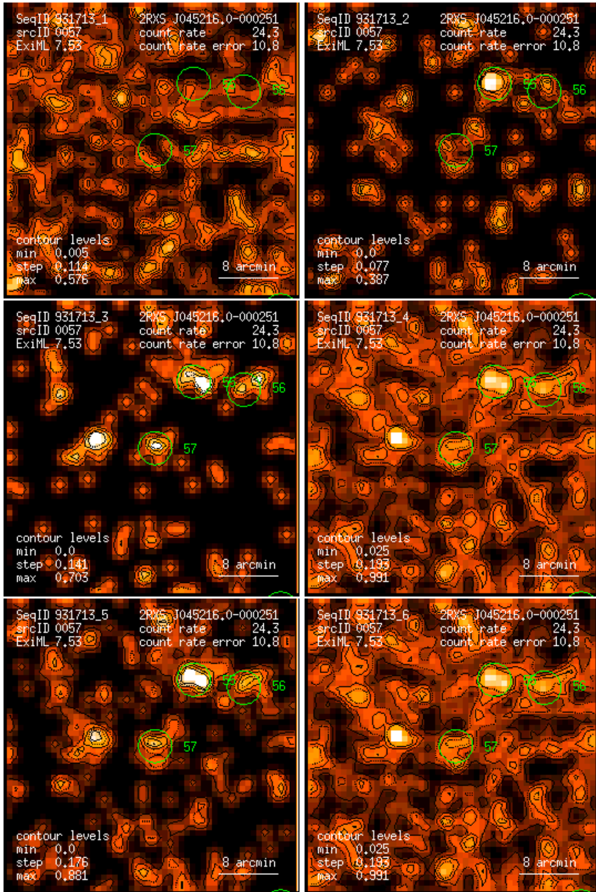
Figure 57: RASS 931713: detection 0057: band rate images, Gaussian filter: (1) PSPC channels 11 – 41, (2) 52 – 90, (3) 91 – 201, (4) 11 – 235, (5) 52 – 201, (6) 11 – 201. Broad band rates in counts/ks. Band rate contour levels in counts/ks/arcmin 2 .
