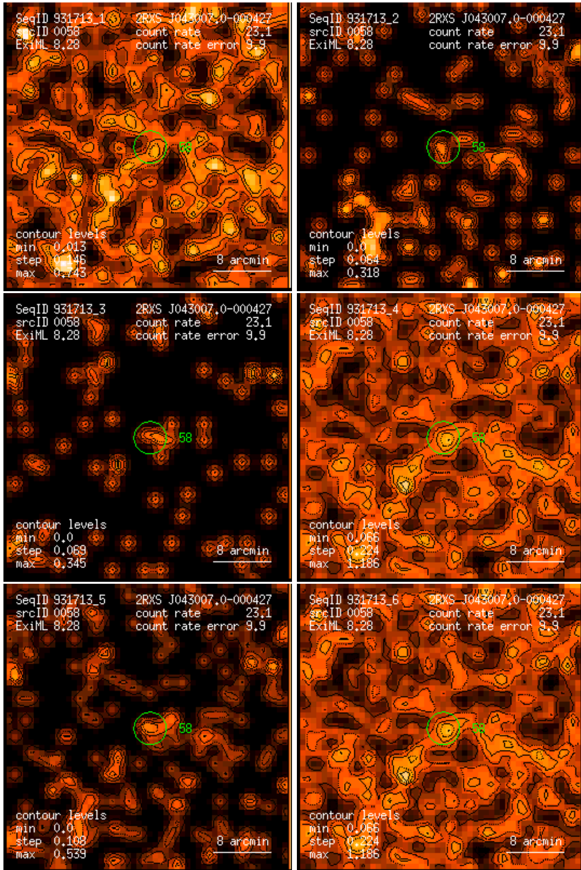
Figure 58: RASS 931713: detection 0058: band rate images, Gaussian filter: (1) PSPC channels 11 – 41, (2) 52 – 90, (3) 91 – 201, (4) 11 – 235, (5) 52 – 201, (6) 11 – 201. Broad band rates in counts/ks. Band rate contour levels in counts/ks/arcmin 2 .
