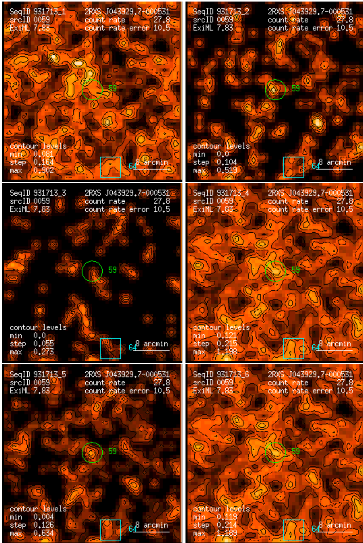
Figure 59: RASS 931713: detection 0059: band rate images, Gaussian filter: (1) PSPC channels 11 – 41, (2) 52 – 90, (3) 91 – 201, (4) 11 – 235, (5) 52 – 201, (6) 11 – 201. Broad band rates in counts/ks. Band rate contour levels in counts/ks/arcmin 2 .
