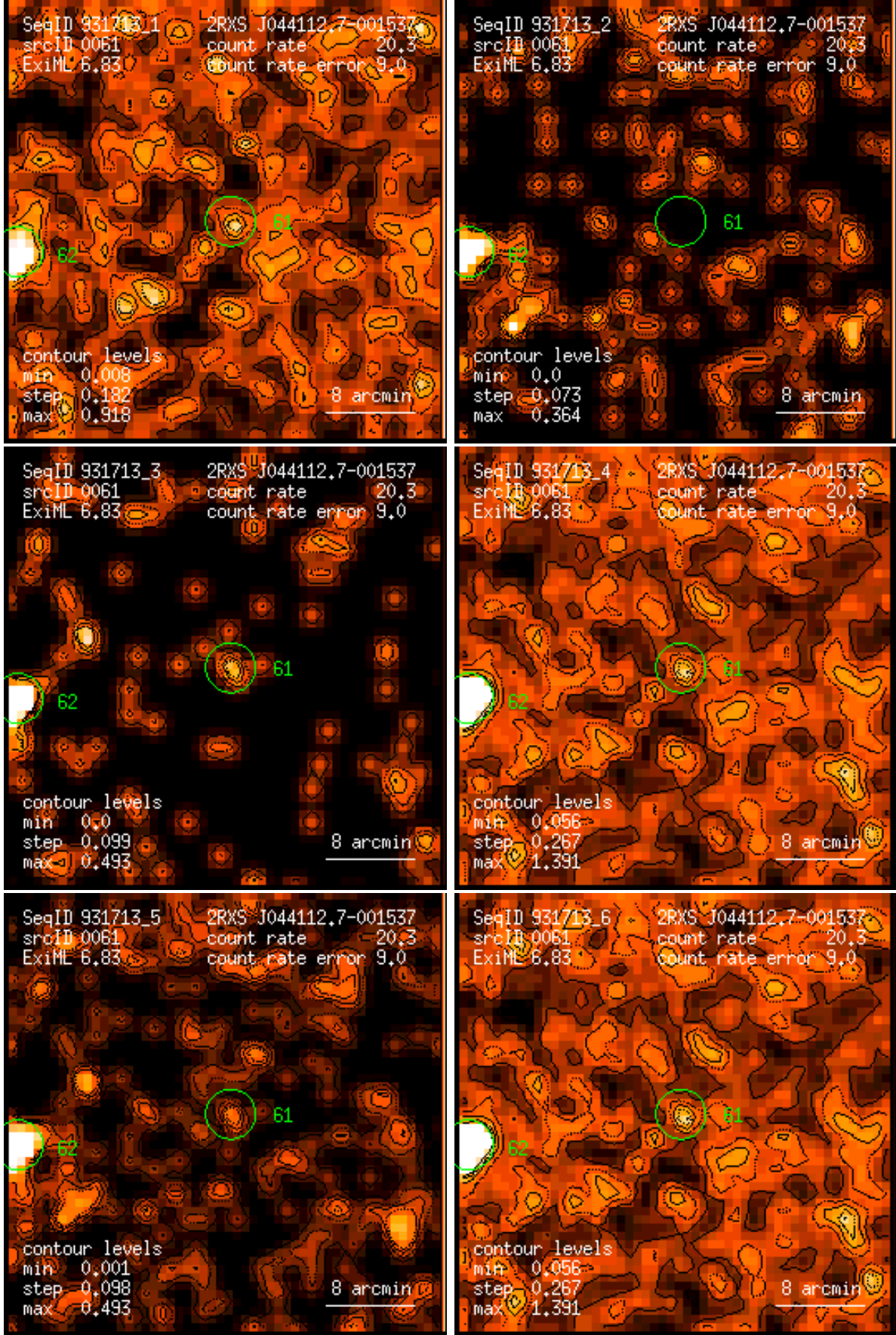
Figure 61: RASS 931713: detection 0061: band rate images, Gaussian filter: (1) PSPC channels 11 – 41, (2) 52 – 90, (3) 91 – 201, (4) 11 – 235, (5) 52 – 201, (6) 11 – 201. Broad band rates in counts/ks. Band rate contour levels in counts/ks/arcmin 2 .
