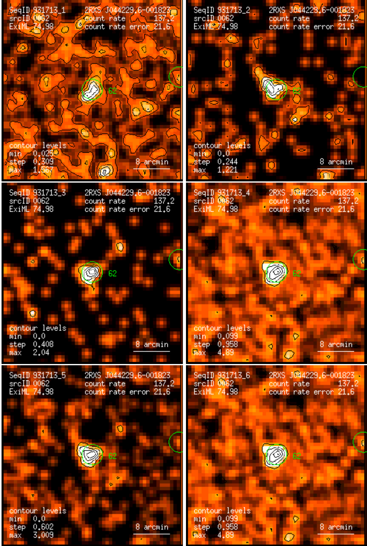
Figure 62: RASS 931713: detection 0062: band rate images, Gaussian filter: (1) PSPC channels 11 – 41, (2) 52 – 90, (3) 91 – 201, (4) 11 – 235, (5) 52 – 201, (6) 11 – 201. Broad band rates in counts/ks. Band rate contour levels in counts/ks/arcmin 2 .
