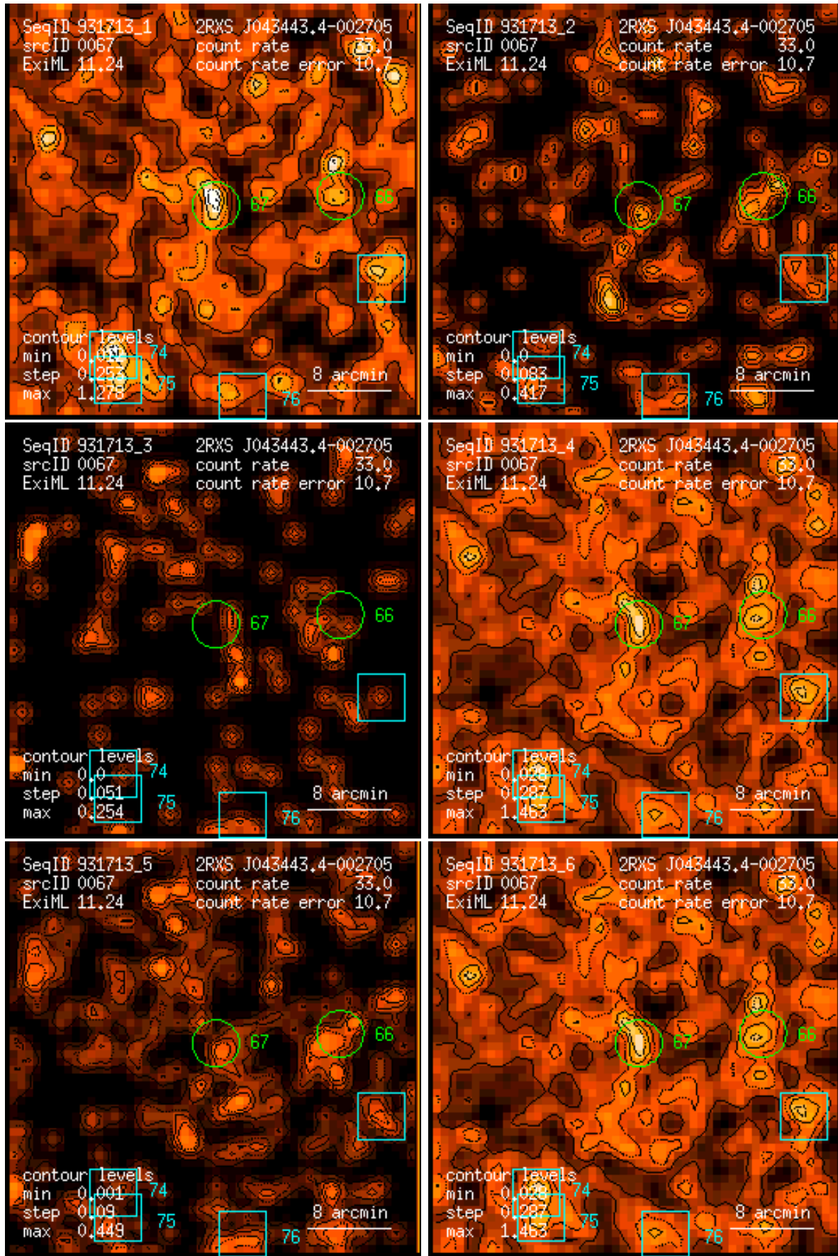
Figure 67: RASS 931713: detection 0067: band rate images, Gaussian filter: (1) PSPC channels 11 – 41, (2) 52 – 90, (3) 91 – 201, (4) 11 – 235, (5) 52 – 201, (6) 11 – 201. Broad band rates in counts/ks. Band rate contour levels in counts/ks/arcmin 2 .
