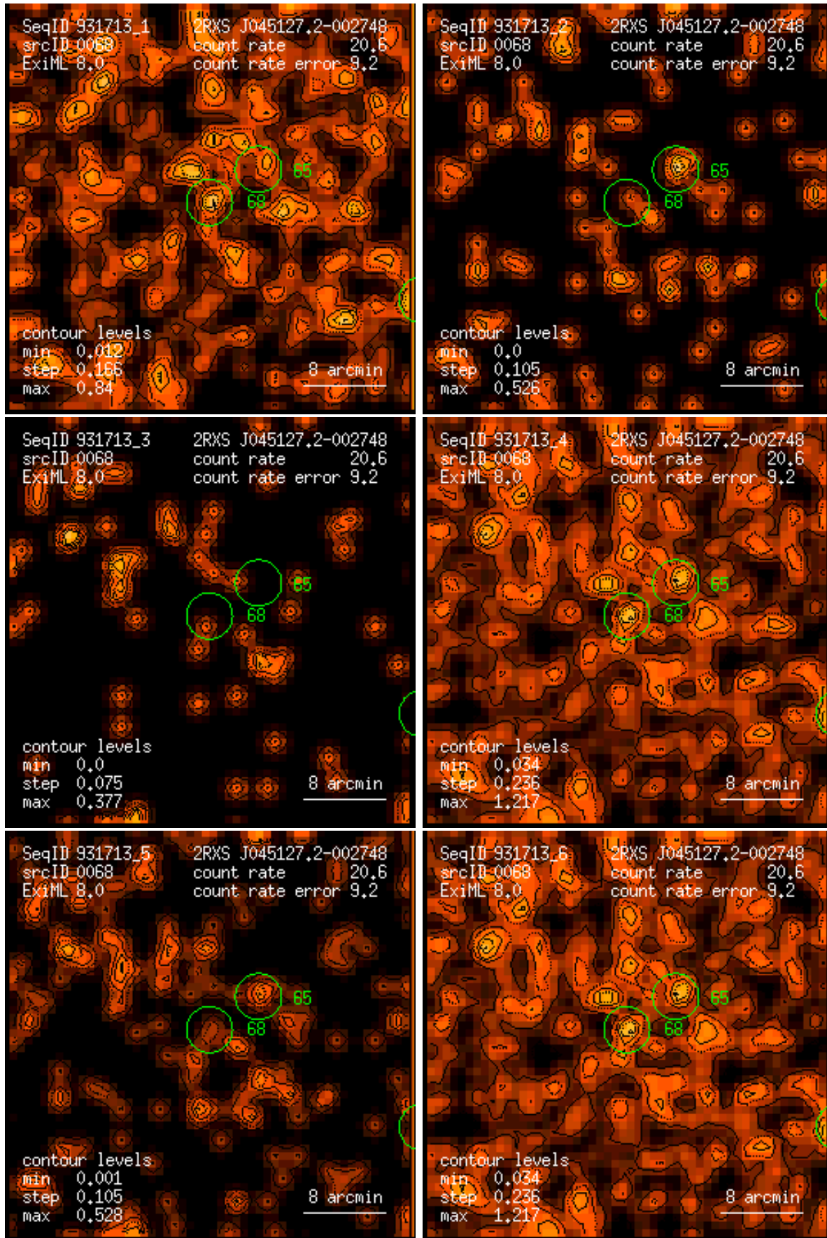
Figure 68: RASS 931713: detection 0068: band rate images, Gaussian filter: (1) PSPC channels 11 – 41, (2) 52 – 90, (3) 91 – 201, (4) 11 – 235, (5) 52 – 201, (6) 11 – 201. Broad band rates in counts/ks. Band rate contour levels in counts/ks/arcmin 2 .
