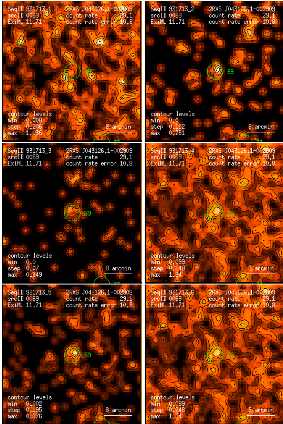
Figure 69: RASS 931713: detection 0069: band rate images, Gaussian filter: (1) PSPC channels 11 – 41, (2) 52 – 90, (3) 91 – 201, (4) 11 – 235, (5) 52 – 201, (6) 11 – 201. Broad band rates in counts/ks. Band rate contour levels in counts/ks/arcmin 2 .
