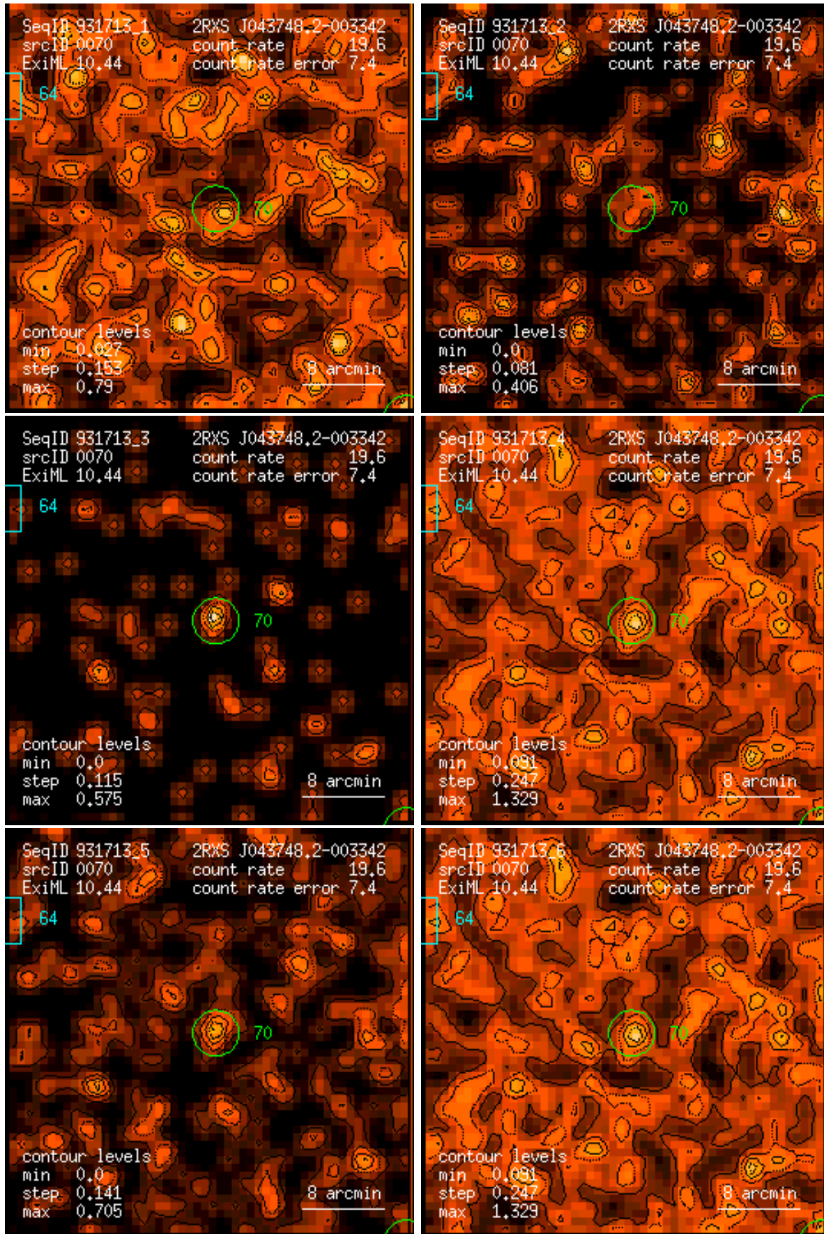
Figure 70: RASS 931713: detection 0070: band rate images, Gaussian filter: (1) PSPC channels 11 – 41, (2) 52 – 90, (3) 91 – 201, (4) 11 – 235, (5) 52 – 201, (6) 11 – 201. Broad band rates in counts/ks. Band rate contour levels in counts/ks/arcmin 2 .
