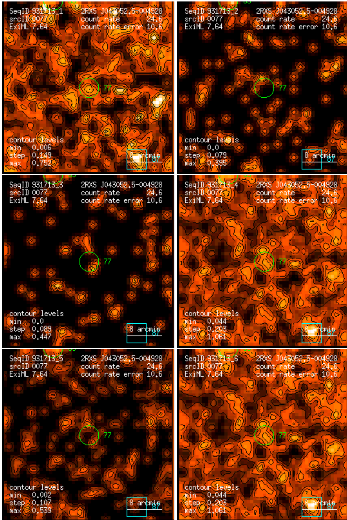
Figure 77: RASS 931713: detection 0077: band rate images, Gaussian filter: (1) PSPC channels 11 – 41, (2) 52 – 90, (3) 91 – 201, (4) 11 – 235, (5) 52 – 201, (6) 11 – 201. Broad band rates in counts/ks. Band rate contour levels in counts/ks/arcmin 2 .
